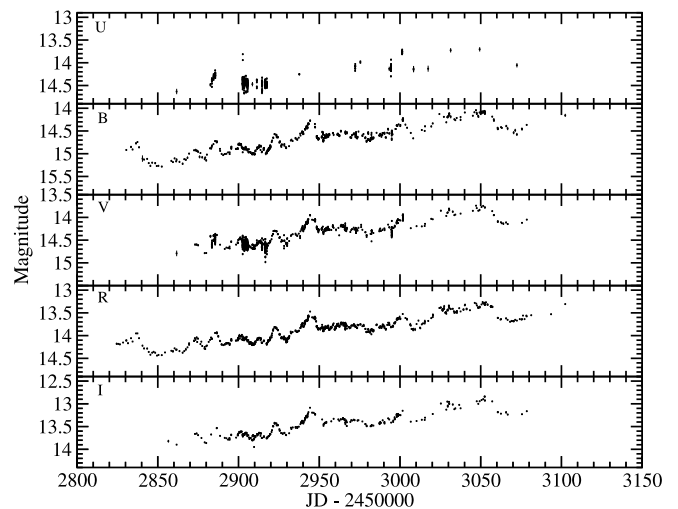
FIG. 6.—Light curves in the optical UBVR bands over the entire duration of the campaign.
