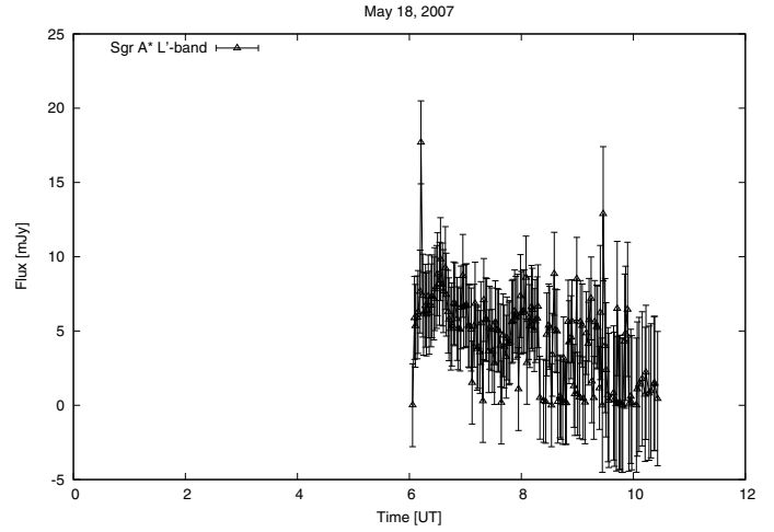
Fig. A.4. Observing time- L' -band: 06:03:26 to 10:26:00.
