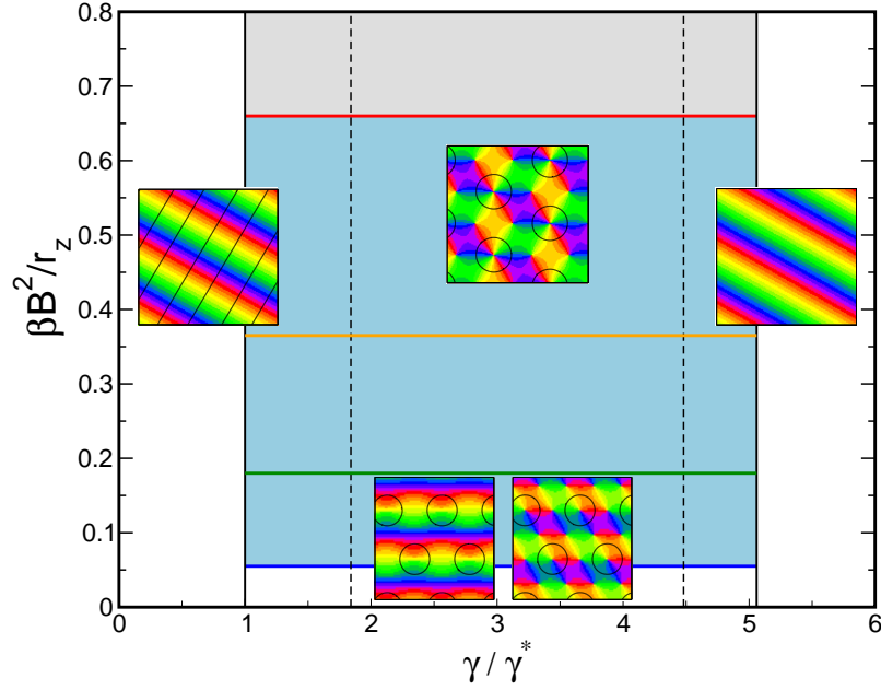
Figure 6. Phase diagram with the coupling energy U = \beta|\nabla\mathbf{z}\cdot\nabla\mathbf{o}|^2 , r_z \ll r_o . Vertical black lines: stability range of OD stripes, hexagons, and constant solution. Blue line: stability border for the \Delta = 0 uniform solution. Green line: rhombic solutions become unstable. Orange line: stripe-like solutions become unstable. Red line: pattern solutions cease to exist, see Eq. (61). Gray region: No pattern solution exists.
