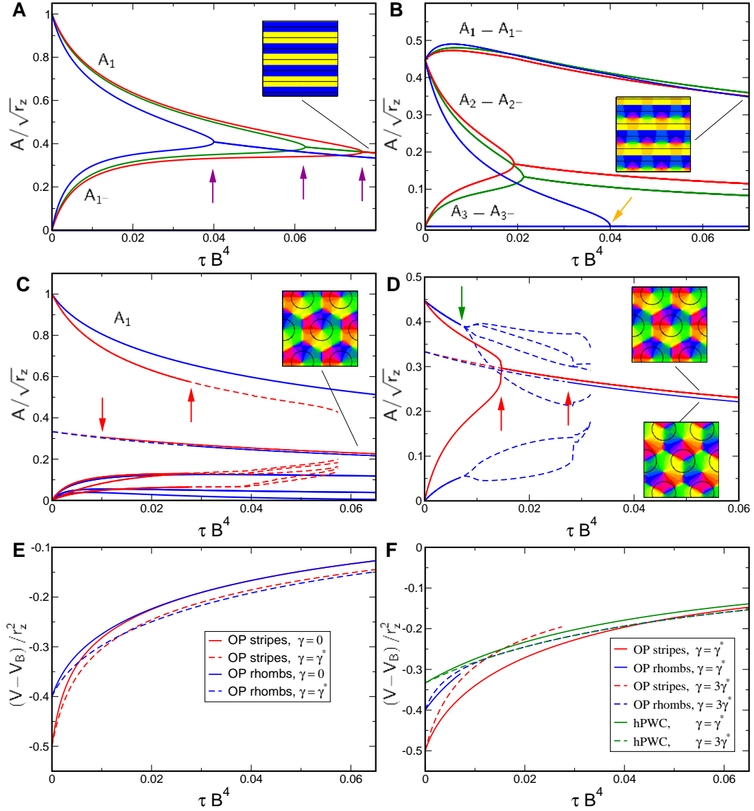
Figure 10. Stationary amplitudes with coupling energy U = \tau|z|^4 \mathbf{o}^4 . Solid (dashed) lines: stable (unstable) solutions. A,B OD stripes, \gamma = 0 (blue), \gamma = \gamma^* (green), \gamma = 1.4\gamma^* (red). C,D OD hexagons, \gamma = \gamma^* (blue), \gamma = 3\gamma^* (red). A,C Transition from OP stripe solutions, B,D Transition from OP rhombic solutions. E Potential, Eq. (125), of OP stripes and OP rhombs interacting with OD stripes. F Potential, Eq. (125), of OP stripes, OP rhombs, and hPWC interacting with OD hexagons. Arrows indicate corresponding lines in the phase diagram, Fig. (11).
