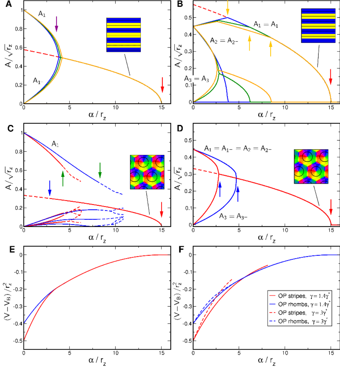
Figure 2. Stationary amplitudes with coupling energy U = \alpha |z|^2 o^2 , r_o = 0.2 . Solid (dashed) lines: stable (unstable) solutions to Eq. (42) (OD stripes) and Eq. (51) (OD hexagons). A,B OD stripes, \gamma = 0 (blue), \gamma = \gamma^* (green), \gamma = 1.4\gamma^* (orange). C,D OD hexagons, \gamma = 1.4\gamma^* (blue), \gamma = 3\gamma^* (red). A,C Transition from OP stripe solutions, B,D Transition from OP rhombic solutions. E Potential for OP stripes (red) and OP rhombs (blue) interacting with OD stripes, \gamma = 0 . F Potential for OP stripes and OP rhombs interacting with OD hexagons. Arrows indicate corresponding lines in the phase diagram, Fig. (3).
