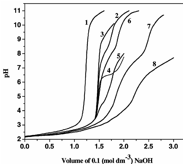
Figure 1. Representative pH titration curves ( M = \text{mol}\cdot\text{dm}^{-3} ): 1, 0.005 (M) \text{HNO}_3 ; 2, (1) + 0.001 (M) \text{H}_2\text{Gu}^+ ; 3, (1) + 0.001 (M) \text{H}_2\text{Gly}^+ ; 4, (2) + 0.001 (M) \text{Cu}^{\text{II}} ; 5, (3) + 0.001 (M) \text{Cu}^{\text{II}} ; 6, (2) + 0.0002 (M) \text{Cu}^{\text{II}} ; 7, (5) + 0.001 (M) \text{H}_2\text{Gu}^+ ; 8, (2) + 0.002 (M) \text{H}_2\text{Gly}^+ + 0.002 (M) \text{Cu}^{\text{II}} ; initial volume = 0.025 \text{ dm}^3 , titrant = 0.1 (M) \text{NaOH} , ionic strength, I = 0.1 \text{ mol}\cdot\text{dm}^{-3} ( \text{NaNO}_3 ).
