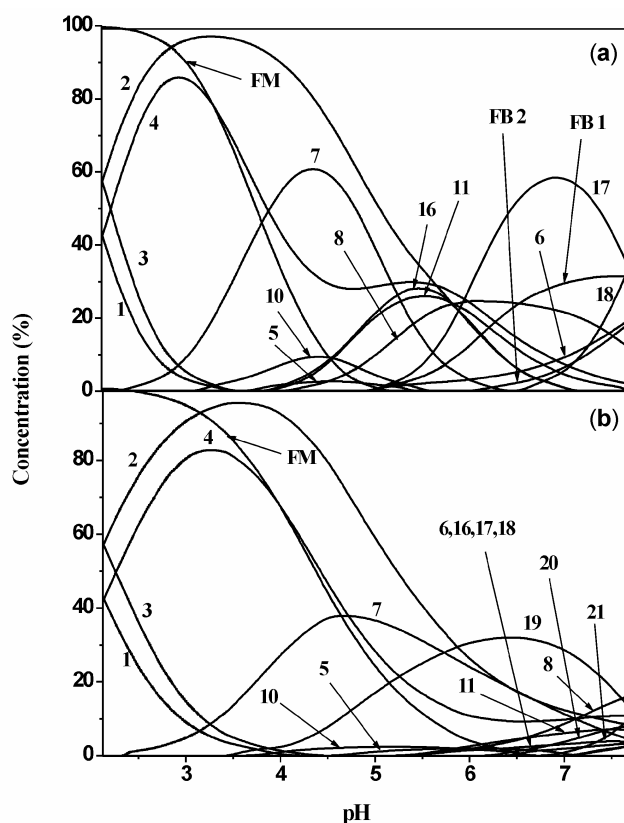
Figure 3. Speciation curves of (a) 1:1:1 and (b) 2:1:2 \text{Cu}^{\text{II}}:\text{GuH}:\text{GlyH} systems: 1, \text{H}_2\text{Gu}^+ ; 2, \text{HGu} ; 3, \text{H}_2\text{Gly}^+ ; 4, \text{HGly} ; 5, \text{Cu}(\text{OH})^+ ; 6, \text{Cu}(\text{OH})_2 ; 7, \text{Cu}(\text{Gly})^+ ; 8, \text{Cu}(\text{Gly})(\text{OH}) ; 10, \text{Cu}(\text{Gu})^+ ; 11, \text{Cu}(\text{Gu})(\text{OH}) ; 16, \text{Cu}(\text{Gly})(\text{Gu}) ; 17, \text{Cu}(\text{Gly})(\text{Gu-H})^- ; 18, \text{Cu}(\text{Gly})(\text{Gu-2H})^{2-} ; 19, (\text{Gly})\text{Cu}(\text{Gu})\text{Cu}(\text{Gly})^+ ; 20, (\text{Gly})\text{Cu}(\text{Gu-H})\text{Cu}(\text{Gly})^- ; 21, (\text{Gly})\text{Cu}(\text{Gu-2H})\text{Cu}(\text{Gly})^- ; FM = Free \text{Cu}^{\text{II}} ; FB1 = Free \text{Gu}^- ; FB2 = Free \text{Gly}^- .
