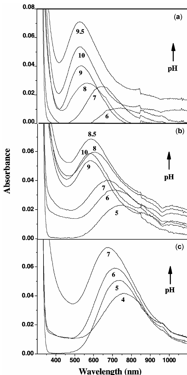
Figure 4. Electronic spectral curves of (a) 1:5 Cu II :GuH; (b) 1:1:1 Cu II :GuH:GlyH; (c) 2:1:2 Cu II :GuH:GlyH mixtures at different pH. Ionic strength, I = 0.1 \text{ mol dm}^{-3} (NaNO 3 ).
