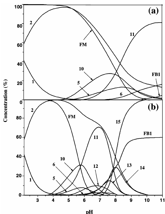
Figure 2. Speciation curves of (a) 1:1 and (b) 1:5 \text{Cu}^{\text{II}}:\text{GuH} systems: 1, \text{H}_2\text{Gu}^+ ; 2, \text{HGu} ; 5, \text{Cu}(\text{OH})^+ ; 6, \text{Cu}(\text{OH})_2 ; 10, \text{Cu}(\text{Gu})^+ ; 11, \text{Cu}(\text{Gu})(\text{OH}) ; 12, \text{Cu}(\text{Gu})_2 ; 13, \text{Cu}(\text{Gu})(\text{Gu-H})^- ; 14, \text{Cu}(\text{Gu-H})_2^{2-} ; 15, \text{Cu}(\text{Gu-H})(\text{Gu-2H})^{3-} ; FM = Free \text{Cu}^{\text{II}} , FB1 = Free \text{Gu}^- .
