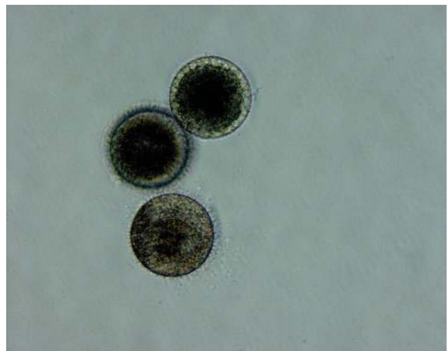
Figure 1. Subitaneous eggs ( \sim 80 \mu\text{m} in diameter) from the calanoid copepod Acartia tonsa Dana.
