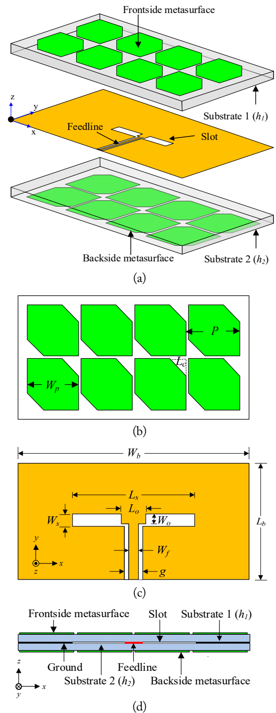
Fig. 1. (a) A 3D-view of antenna, (b) truncated 2 \times 4 front/side metasurface patches, (c) slot etched on ground plane, and (d) side view.
