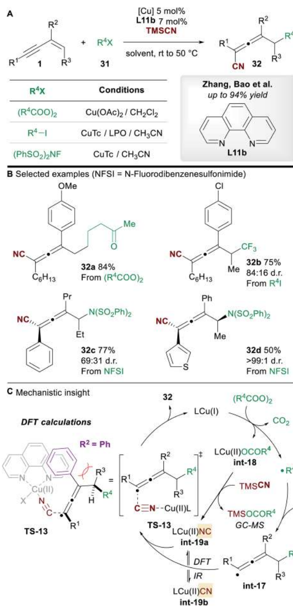
Scheme 19 Zhang and Bao's carbocyanation of 1,3-enynes. NFSI = N -fluorobenzenesulfonimide.
