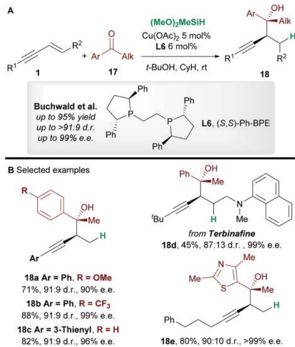
Scheme 11 Buchwald's hydrofunctionalization of 1,3-enynes with ketones.
