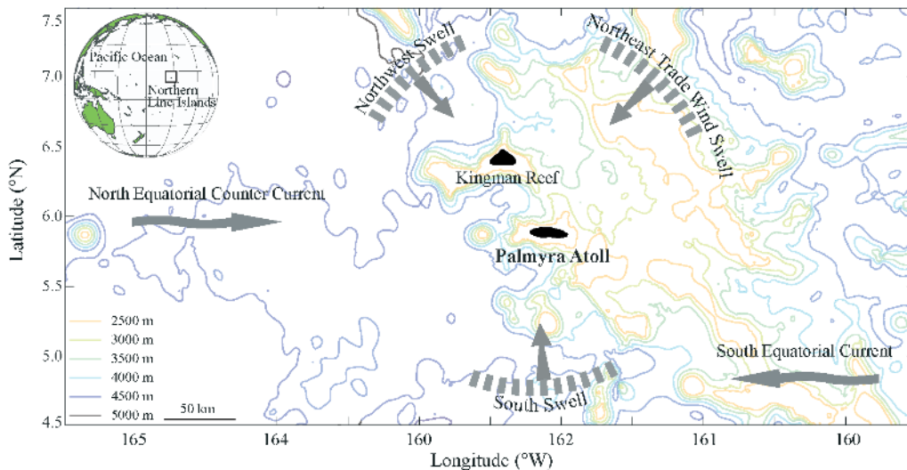
Fig. 1. US-owned atolls in the northern Line Islands of the central Pacific (inset globe), highlighting the dominant wave regimes, regional currents, and seafloor bathymetry
