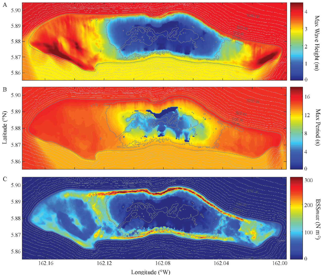
Fig. 4. Hydrodynamic wave model results representing the maximum values of (A) significant wave height, (B) wave period, and (C) bed shear stress ( \text{BSS}_{\text{max}} ) at Palmyra Atoll. Results represent the maximum of each grid cell from the combined hydrodynamic model runs for each swell regime (i.e. northwest swell, northeast trade wind swell, and south swell) at Palmyra Atoll (see Fig. 1)
