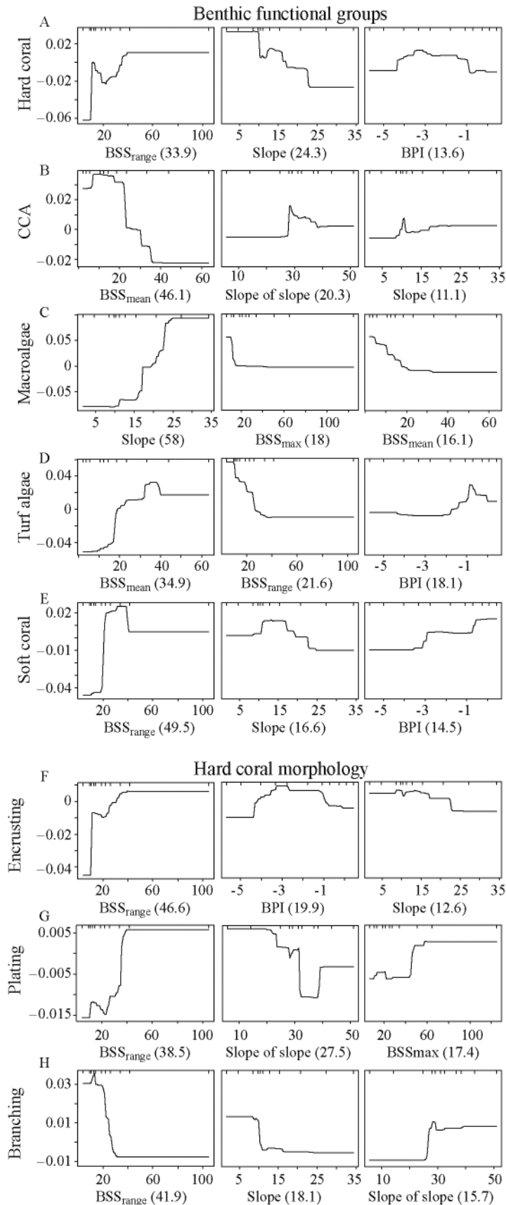
Fig. 6. Partial dependency response plots from boosted regression tree analyses for the 3 most influential predictors of variations in the percent cover of 5 dominant benthic functional groups: (A) hard coral, (B) crustose coralline algae (CCA), (C) macroalgae, (D) turf algae, and (E) soft coral; and 3 dominant hard coral morphologies: (F) encrusting, (G) plating, and (H) branching. Relative influence of each variable is given in parentheses after the x-axis label. The y-axes are on logit scale and are centered to have zero mean over the data distribution. Tick marks along the inside top of each subpanel indicate the distribution of the replication for that variable (e.g. hard coral) across the corresponding predictor (e.g. slope). BPI: bathymetric position index; BSS_{max} , BSS_{mean} , BSS_{range} : bed shear stress maximum, mean, and range, respectively
