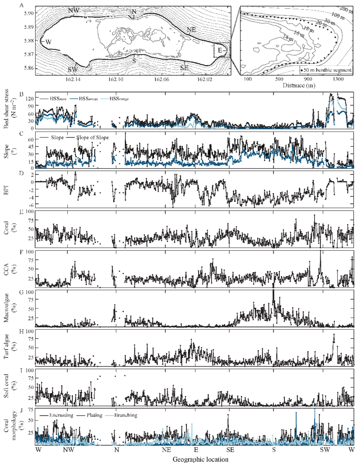
Fig. 5. (A) Bathymetric map of Palmyra Atoll (left) with an expanded section (right) showing depth-constrained (15–20 m) and spatially averaged 50 m benthic segments collected via towed-diver surveys (black filled circles). (B–J) Corresponding wave, geomorphology, and coral reef benthic community data for each 50 m segment. Note the x-axis ('Geographic location') corresponds to (A, top left), showing all data in a clockwise fashion from left to right, starting at the western tip of the atoll (W) and moving northwest (NW), north (N), northeast (NE), east (E), southeast (SE), south (S), southwest (SW), and ending back at the western tip. (B) Bed shear stress (maximum, mean, and range), (C) slope (and slope of slope), (D) bathymetric position index (BPI), and percent cover of (E) hard coral, (F) crustose coralline algae (CCA), (G) macroalgae, (H) turf algae, (I) soft coral, (J) variations in the 3 most dominant hard coral morphologies (encrusting, plating, branching)
