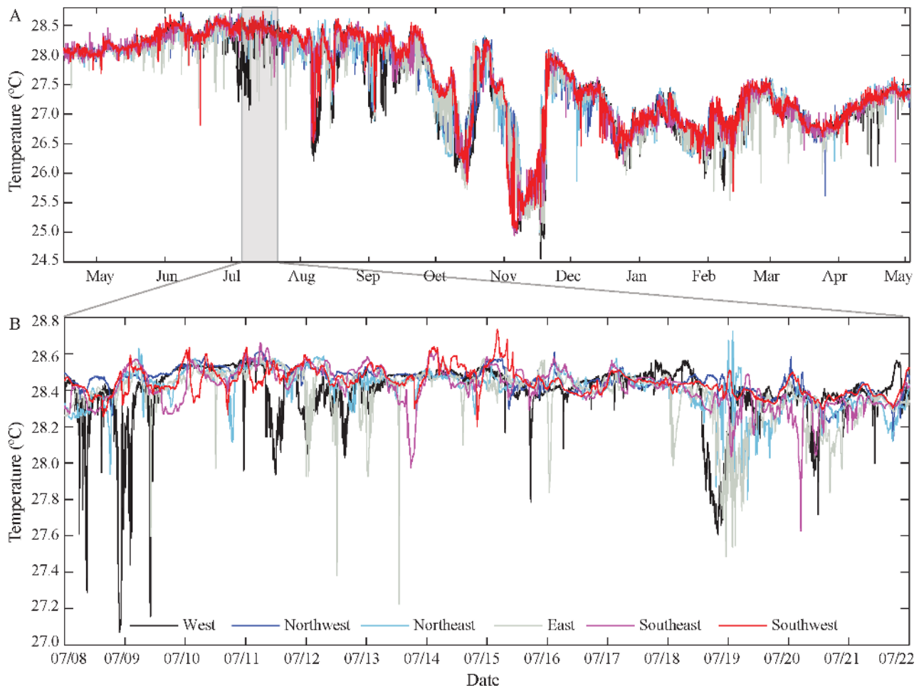
Fig. 3. (A) In situ time series data of temperature from 6 mooring locations deployed at ~20 m depth from April 2010 to May 2011. (B) Two-week expansion of temperature data highlighting the high-frequency temperature drops observed at all locations. Legend in (B) corresponds to both panels. See Fig. 2 for individual mooring locations
