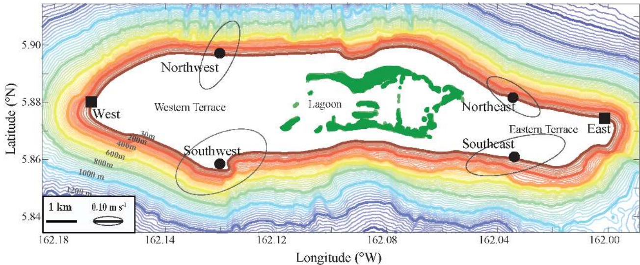
Fig. 2. Palmyra Atoll, showing the 6 mooring locations where oceanographic time series data were collected along the ~20 m isobath. ●: moorings where profiling currents, waves and temperature data were collected; ■: moorings where only temperature data were collected. Current variance ellipses represent the magnitude ( \pm 1 SD from mean current flow) and orientation of near-bottom currents. The scale bar for current magnitude is also given ( 0.10 \text{ m s}^{-1} )
