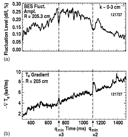
FIG. 10. (a) Fluctuation amplitude ( \tilde{n}_e/n_e ) versus time from the BES diagnostic for a shot with confinement improvement at the time of q_{\min}=3 and q_{\min}=2 crossings. (b) Local T_e gradient versus time at the BES measurement radius. The radius of the q_{\min} is between 200 and 205 cm for this time window.
