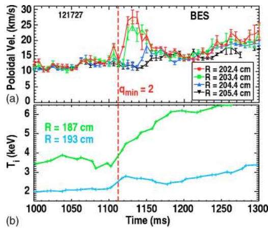
FIG. 11. (a) Poloidal velocity evolution derived from BES measurements near the q_{min}=2 time for the same discharge as Fig. 10. (b) Core T_i versus time for two locations showing barrier formation at the q_{min}=2 crossing.
