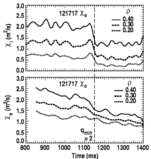
FIG. 13. Core ion and electron diffusivities versus time from TRANSP for the discharge of Fig. 1 showing the stepwise change in confinement in the ion channel at the q_{min}=2 time, but no similar step in the electron channel.
