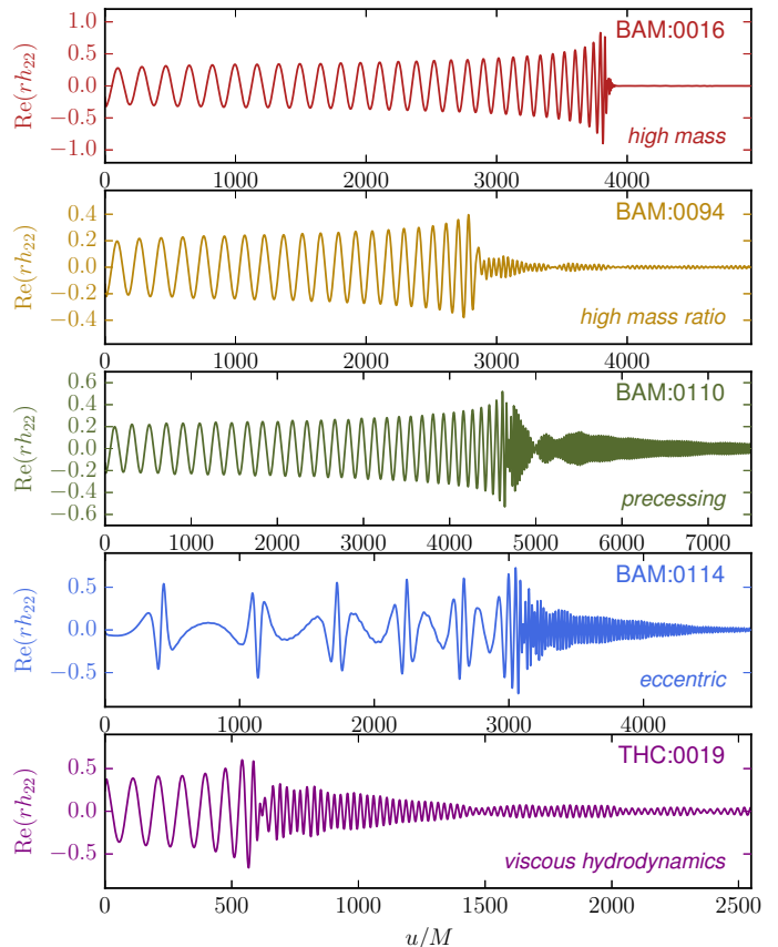
FIG. 2. Waveforms from the database showing, from top to bottom panel, the influence of total mass, mass ratio, spins, eccentricity, and EOS.
