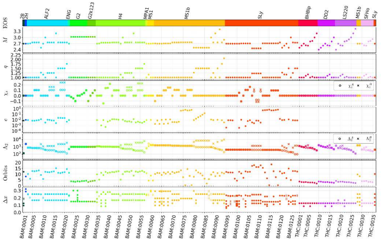
FIG. 1. Simulations contained in the CoRe database. We present the total mass M , the mass ratio q , the individual dimensionless spins \chi_z^{A,B} , the eccentricity e [no eccentricity measurement is given for too short simulations], the individual quadrupolar tidal parameters \Lambda_2^{A,B} , the number of orbits [note that for highly eccentric orbits close to head-on, the number of orbits can drop below 1], and the employed resolution \Delta x of the finest level covering the entire NS for different configurations. Different colored markers refer to different EOS, see top color bar. In the last panel we also include simulations with different grid resolutions and numerical methods (fluxes, mesh refinement strategies etc.); simulations of a fixed configuration performed at the same resolutions but using different methods are marked with vertical bars in this panel.
