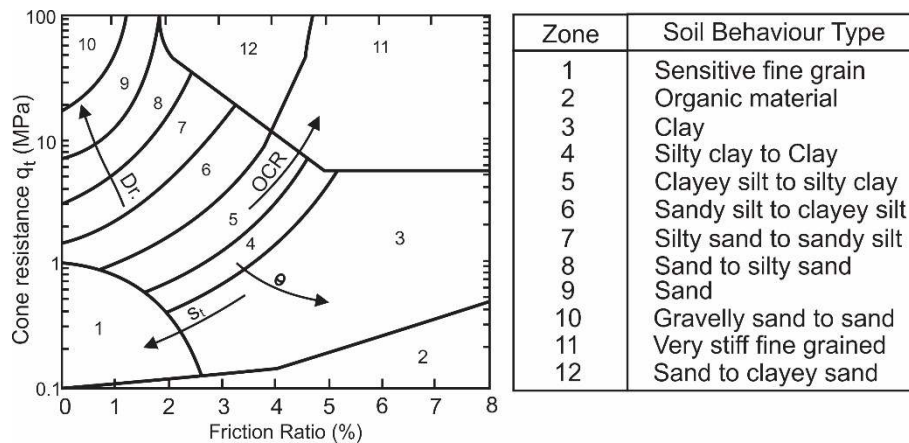
Figure 5: Soil type diagram modification from Lunne et al. (1997)
