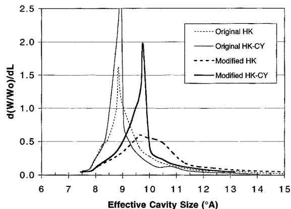
Figure 16. PSD of 5A (Ca-A) zeolite as predicted by original and modified HK models for spherical pores.
