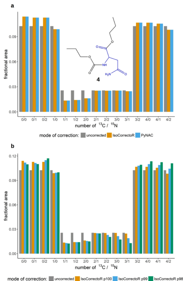
Figure 5. Correction of high-resolution-multiple-tracer data. (a) shows the correction results of simulated high-resolution data of simultaneously ^{13}\text{C} - and ^{15}\text{N} -labeled and PCF-derivatized asparagine (chemical structure 4 in the diagram). The x-axis labels describe the labeling state of the respective species. The first number represents the amount of ^{13}\text{C} , the second (after the slash) the number of ^{15}\text{N} . The group bar charts depict the correction results of IsoCorrectoR and PyNAC and the uncorrected data. (b) is basically analogous to (a) except that it compares the correction results without considering tracer purity (p100) with the correction results at the tracer purities 99% (p99) and 98% (p98). PyNAC results are not included in this diagram as it cannot correct for tracer purity.
