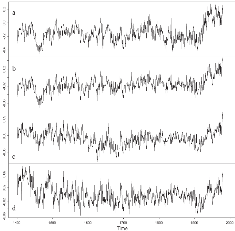
Figure 6. (a) MBH98 NH temperature series (C), 1400-1980, which relies heavily on (b) TPC1 from MBH98. (c) Authors' replication of TPC1 using MBH98 methods and data. (d) Authors' TPC1 using MBH98 methods but with data corrected as outlined in text.
