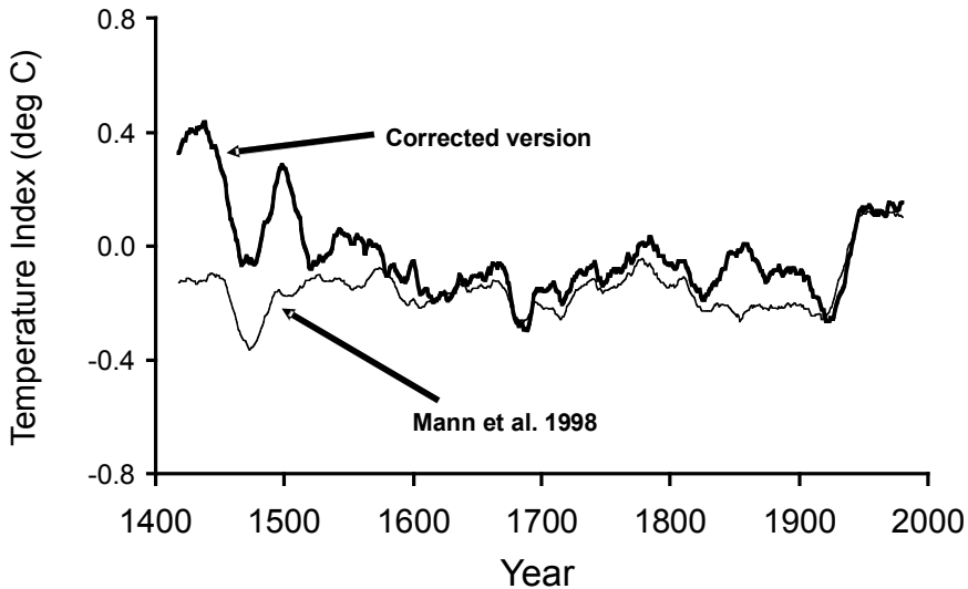
Figure 8. As Figure 7, using 20-year running mean to smooth.
