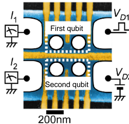
Multi-functional quantum information processing device fabricated by using GaAs/AlGaAs heterostructure (upper left), Simulation of correlated coherent oscillations (upper right)
