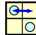
Controlled (blue) and correlated (red) coherent oscillation.
