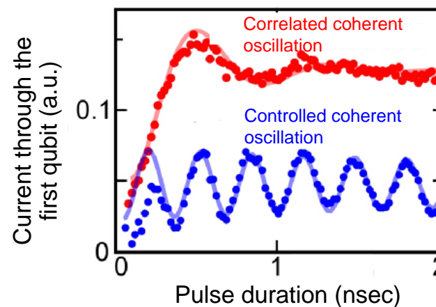
Controlled (blue) and correlated (red) coherent oscillation.
