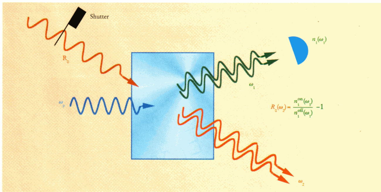
FIGURE 5. SPECTRAL RADIANCE of the photon beam R_0 can be measured at \omega_2 by overlapping it with the crystal along the \omega_2 output direction. The double wavy lines at output frequencies \omega_1 and \omega_2 indicate the enhancement of photon-pair production caused by adding the R_0 input. Energy conservation dictates that \omega_1 + \omega_2 = \omega_p . If one measures the n_1(\omega_1) signal with an uncalibrated detector in a convenient visible region, one can get the absolute radiance of R_0 in the more difficult infrared region \omega_2 simply from the ratio of the visible detector signals with R_0 on and off.
