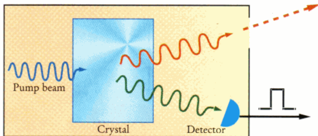
FIGURE 4. NEW ABSOLUTE PHOTON SOURCE exploits the constraints of simultaneity and energy-momentum conservation on pairs of photons produced by down-conversion of pump-beam photons in a nonlinear crystal to specify not only the direction and wavelength of an output photon, but also its time of emission, simply by recording its partner in a detector.
