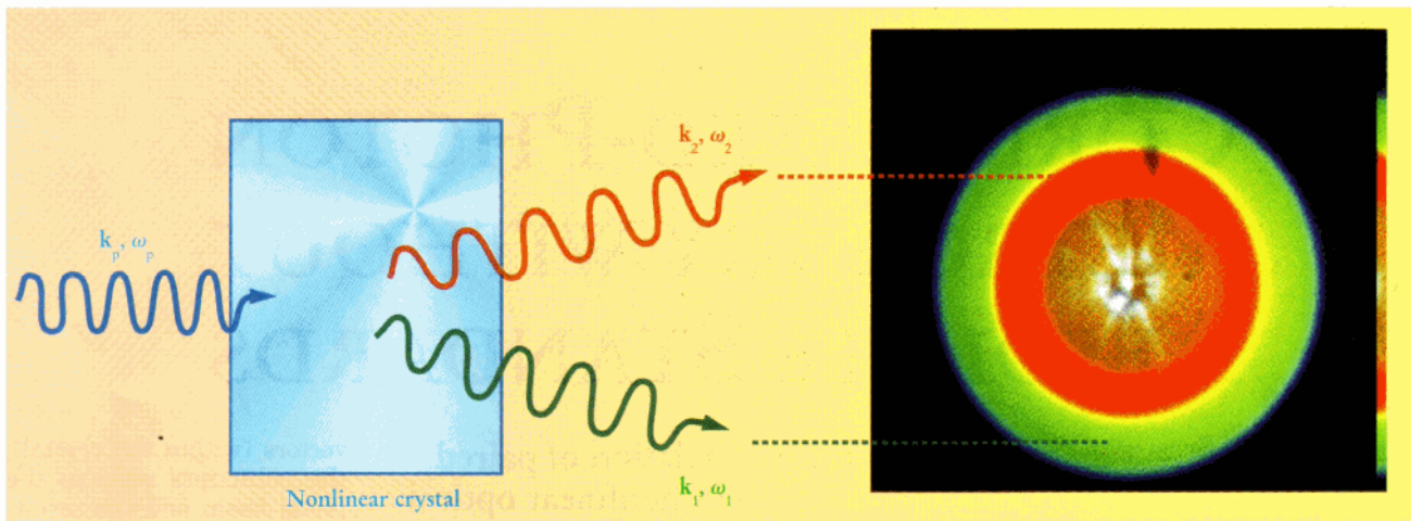
FIGURE 1. PARAMETRIC DOWN-CONVERSION, turning a single photon entering an optically nonlinear crystal into two photons coming out, is essentially the inverse of sum-frequency generation. The energy \hbar\omega and momentum \hbar\mathbf{k} of the incident photon equals the sums of the outgoing energies and momenta. The concentric circles of output light in different colors (at right), azimuthally symmetric about the monochromatic pump-beam axis, indicate the broad spectral range of the down-converted light. At their center, one sees some of the pump light leaking around a beam stop.
