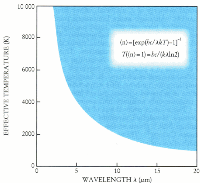
FIGURE 6. EQUIVALENT TEMPERATURE of a blackbody background with a spectral radiance of one photon per mode. Formulas are displayed for the mean number of photons per mode at a given wavelength and temperature as well as for the temperature required for a source to emit, on average, one photon per mode at the given wavelength. ( k is Boltzmann's constant.) The blue region above the curve indicates the regime of wavelengths and temperatures best suited for absolute radiance measurement with correlated photon pairs.
