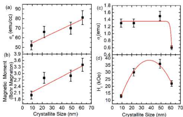
Fig. 5 (a) Saturation magnetization, (b) magnetic moment (c) remnant magnetization and (d) coercivity as a function of crystallite size.
