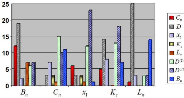
Fig. 3. Number of networks (among the 34 real-world networks) in which M_{A,B}(\gamma) is the highest among the centrality similarities between A and all other centrality metrics, when \gamma = 5\% . The centrality metric A is given by the x -axis label, and B is reflected by the pattern described in the box on right side. Take the betweenness B_n as an example. The centrality similarities between B_n and all the other metrics are compared with each other to find the largest similarity in each real-world network. For instance, the M_{B_n,C_n}(\gamma) is the largest centrality similarity in ‘Electric_s208’ network, so that one is counted into the leftmost bar of B_n (with C_n ).
