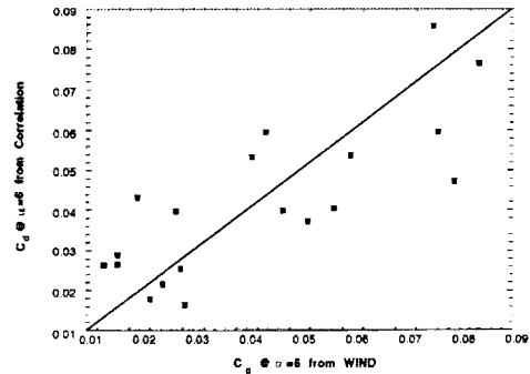
FIGURE 54. Calculated Drag from Regression Equation
