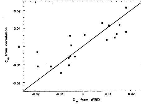
FIGURE 58. Calculated Pitching Moment from Regression Equation
