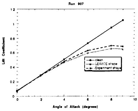
FIGURE 16. Run 907 Lift Comparison
