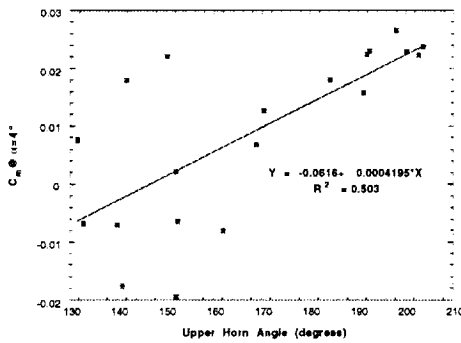
FIGURE 56. Pitching Moment vs. Upper Horn Angle
