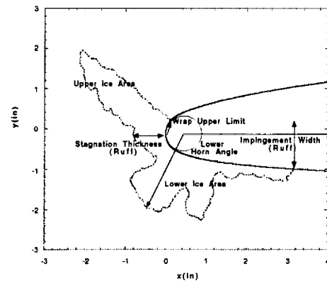
FIGURE 43. Additional Geometric Measurements
