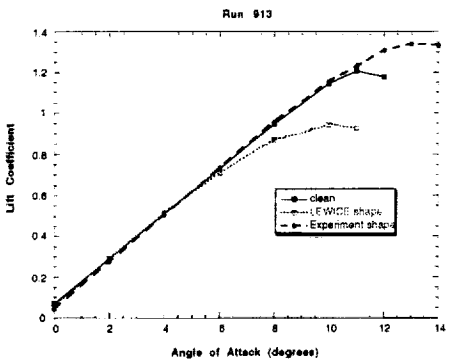
FIGURE 17. Run 913 Lift Comparison
