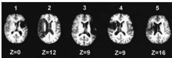
Fig. 1 Location of lesions for patients with cortical strokes (Patients 1–5). Single axial slices in the centre of the lesion volume are shown for illustration. Talairach Z coordinates are given for each slice. Total lesion volume is given in Table 1. No lesions included the hand area of primary motor cortex or the dorsal premotor cortex.
