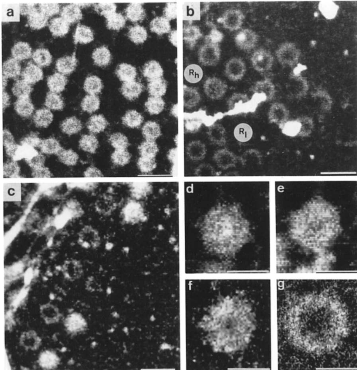
Figure 4. Elastic annular dark-field STEM images of freeze-dried, unstained, and completely unfixed intact ( a , d , and e ) and detergent-treated ( b , c , f , and g ) NPCs digitally recorded at low doses ( 50 to 300\ e^-/\text{nm}^2 ). ( a ) Nuclear envelope with embedded intact NPCs spanning a fissure in the carbon support film. Such “unsupported” areas were used for mass determination. ( b ) Distinct NPC components revealed after detergent treatment of the material shown in ( a ) directly adsorbed to a 4-nm-thick carbon support film. The following structures can be distinguished: “heavy” rings ( R_h ; bright rings), “light” rings ( R_l ; dimmer rings), and “particles” (bright spherical dots, diameter \sim 20 – 35\ \text{nm} ). ( c ) Same preparation as in b depicting “complementary” NPC components consisting of a heavy ring and a plug-spoke or spoke complex. ( d – g ) Higher magnification en face views of an intact NPC with plug ( d ), an intact NPC without plug ( e ), a spoke complex ( f ), and a heavy ring ( g ). Bars, 200 nm ( a – c ), and 100 nm ( d – g ).
