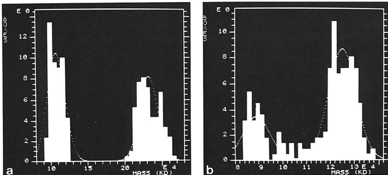
Figure 5. STEM mass histograms of membrane-detached intact NPCs ( a ) and heavy rings ( b ). In both histograms the left peak represents the mass distribution of empty carbon support film, while the right peak represents the mass distribution of particles plus carbon support film. Gaussian profiles were fitted to the experimental mass distributions using a Marquardt fitting algorithm (Bevington, 1969) yielding peak positions as well as standard deviations. The average masses of the intact NPC and the heavy ring are given by the difference of the two peak positions in each histogram.
