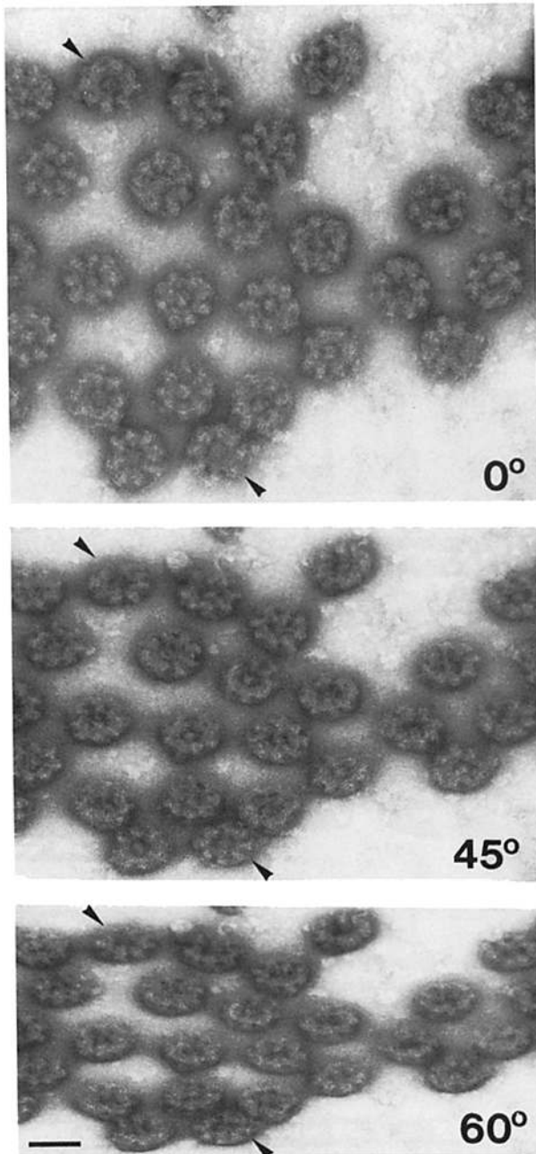
Figure 2. CTEM 0°/45°/60° tilt series of negatively stained detergent-treated NPCs prepared and processed as described in Fig. 1. Two representative particles have been identified with arrowheads throughout the tilt series. From the tilted views it becomes obvious that the detergent-treated NPCs are devoid of rings. As in Fig. 1, each micrograph within the tilt series was recorded under low-dose conditions ( \leq 2,000 e - /nm 2 ). Bar, 100 nm.
