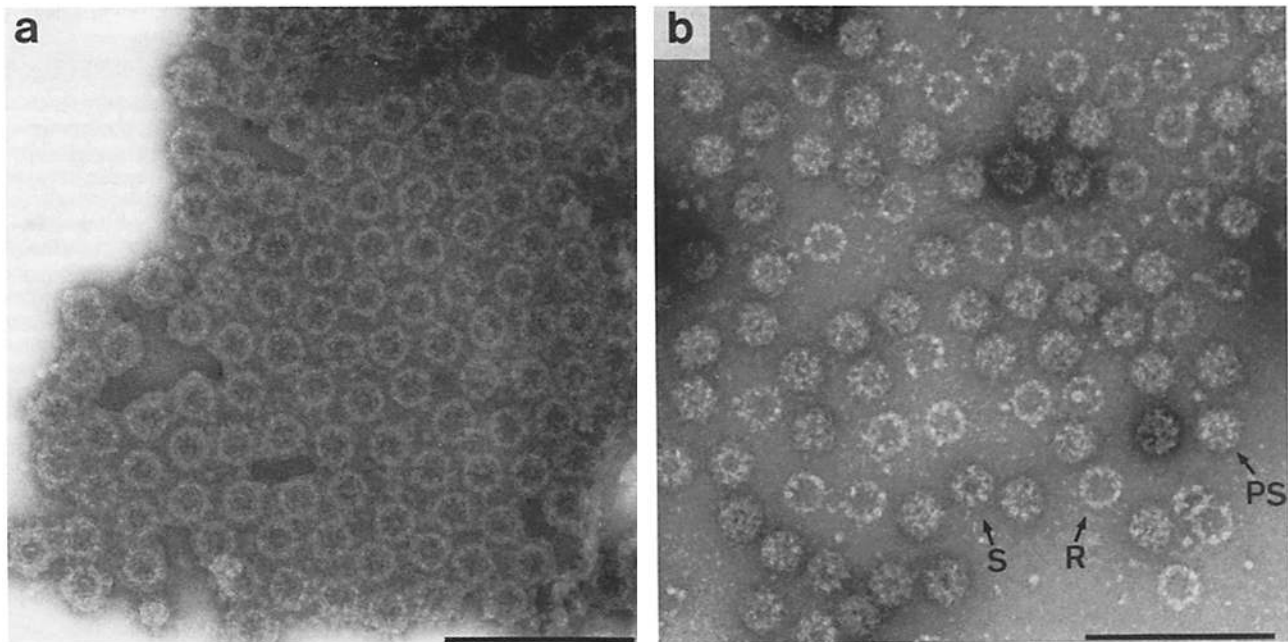
Figure 1. CTEM images of negatively stained intact ( a ) and detergent-treated ( b ) NPCs prepared from spread nuclear envelopes manually isolated from Xenopus laevis oocytes. Whereas the intact NPCs in a are embedded in the nuclear envelope, the detergent-treated NPCs in b have detached from the nuclear envelope and are directly adsorbed to the support film. As illustrated in b , detergent treatment leads to disintegration of the intact NPCs into three distinct NPC components, i.e., plug-spoke complexes (PS), spoke complexes (S), and rings (R). Both preparations ( a and b ) were processed without OsO 4 fixation and negatively stained with 0.75% uranyl formate, pH 4.25. To minimize beam-induced radiation damage, all micrographs were recorded under low-dose conditions ( \leq 2,000 e - /nm 2 ). Bars, 500 nm ( a and b ).
