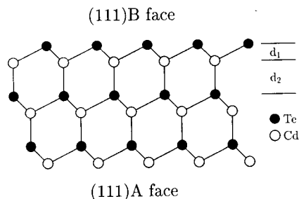
FIG. 3. Crystal structure of (111) CdTe: \circ , Cd; \bullet , Te.
