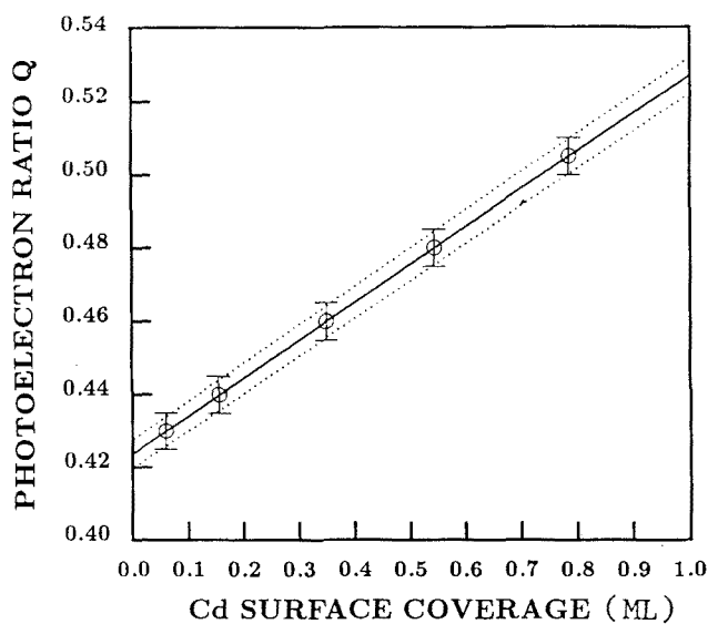
FIG. 4. The theoretical Cd fraction on the (100) CdTe surface vs the photoelectron-intensity ratio as measured by x-ray photoelectron spectroscopy.
