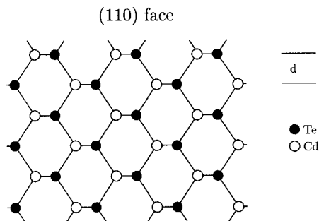
FIG. 2. Crystal structure of (110) CdTe: \circ , Cd; \bullet , Te.
