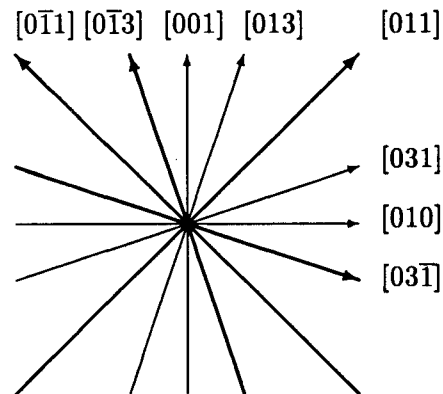
FIG. 1. The azimuths in which reconstruction can be observed in reflection high-energy electron-diffraction patterns of the (100) CdTe surface. The azimuths for a Te and Cd environment are indicated by thick and thin lines, respectively.
