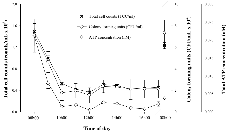
Figure 2. Daily changes of total cell counts (TCC), colony forming units (CFU) and total adenine tri-phosphate (ATP) concentration for one representative drinking water tap, sampled on a normal working day. Error bars indicate the standard deviation on triplicate measurements.
