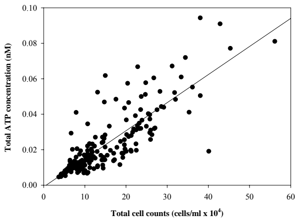
Figure 3. Correlation between total ATP concentrations and total cell concentrations of all samples ( n=200 ). All data points represent average values of triplicate measurements.
