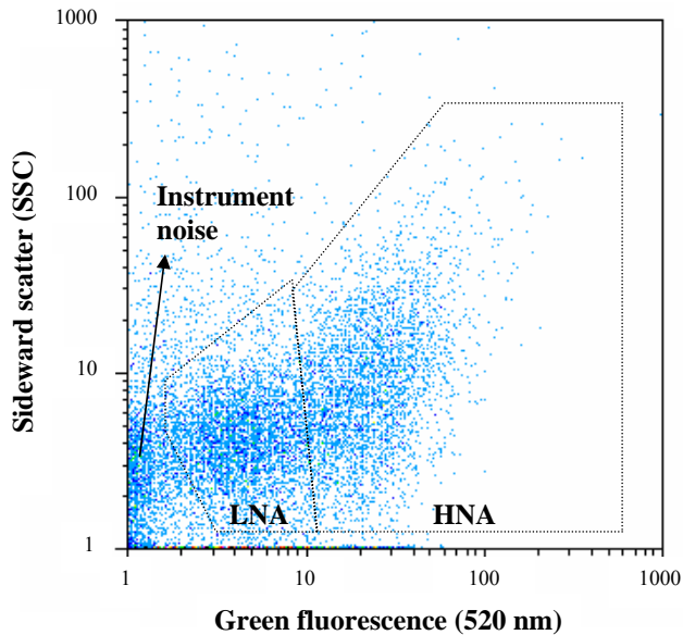
Figure 1. A 2-dimensional flow cytometry dot-plot of green fluorescence (520 nm) and sideward scattered light (SSC), distinguishing so-called high nucleic acid (HNA) and low nucleic acid (LNA) content bacteria.
