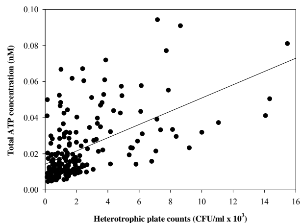
Figure 4. Correlation between total ATP concentrations heterotrophic plate counts (HPC) of all samples ( n=200 ). All data points represent average values of triplicate measurements.
