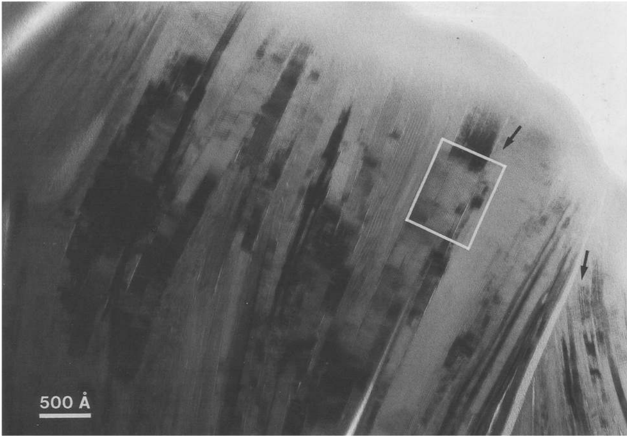
Fig. 5. TEM bright field image of the amygdule core material showing that packets of mixed-layer chlorite/corrensite are 100 to 500 Å thick. Most layers are 14 Å chlorite layers but some interstratified
