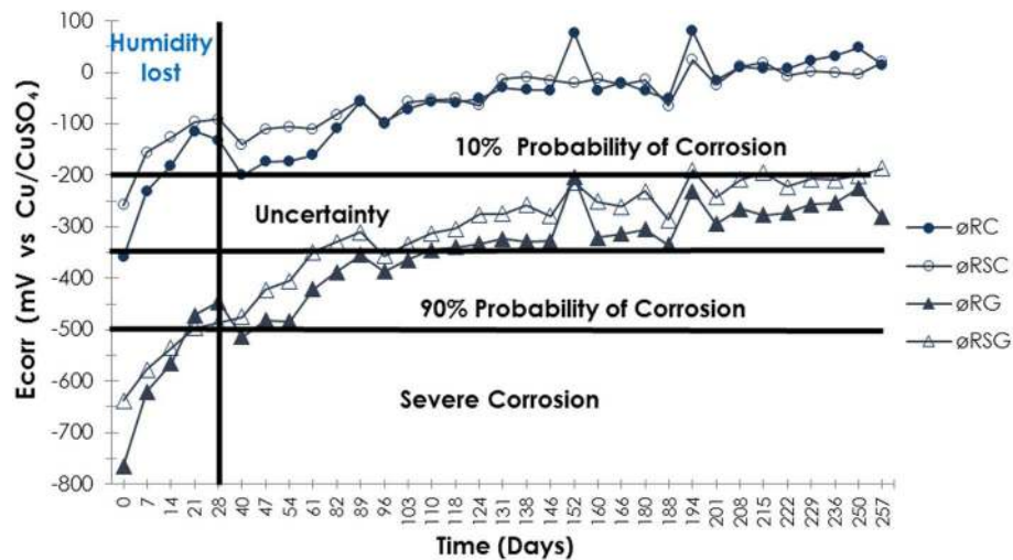
FIGURE 3 | E_{\text{corr}} specimens in soil type MH with 0% of NaCl.
