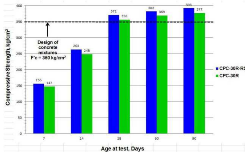
FIGURE 1 | Compressive strength concrete mixtures CPC 30R RS and CPC 30R.
