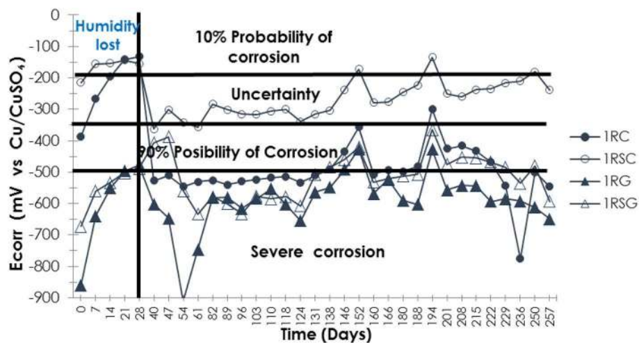
FIGURE 4 | E_{\text{corr}} specimens in soil type MH with 1% of NaCl.
