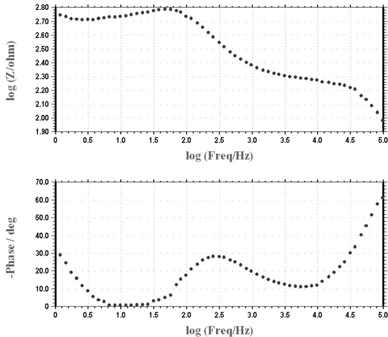
Figure 2c. AC impedance spectra of aluminium immersed in aqueous solution at pH 12 (NaOH). Bode plots: (c) aqueous solution at pH 12.
