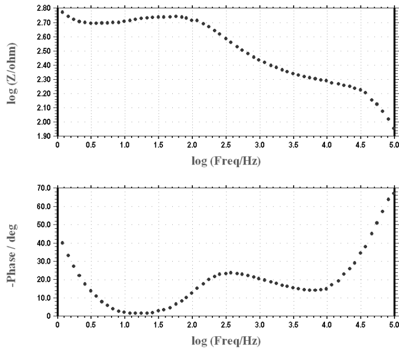
Figure 2d. AC impedance spectra of aluminium immersed in aqueous solution at pH 12 (NaOH). Bode plots: (d) flower extract 8 mL + Zn^{2+} 50 ppm (pH 12).
