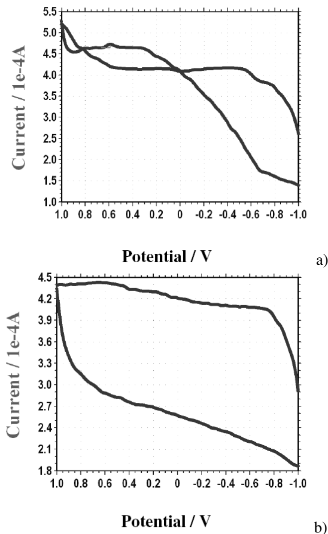
Figure 3. Cyclic voltammograms of aluminium immersed in aqueous solution at pH 12 (NaOH). (a) Aqueous solution at pH 12; (b) (b) Flower extract 8 mL + Zn 2+ 50 ppm (pH 12).
