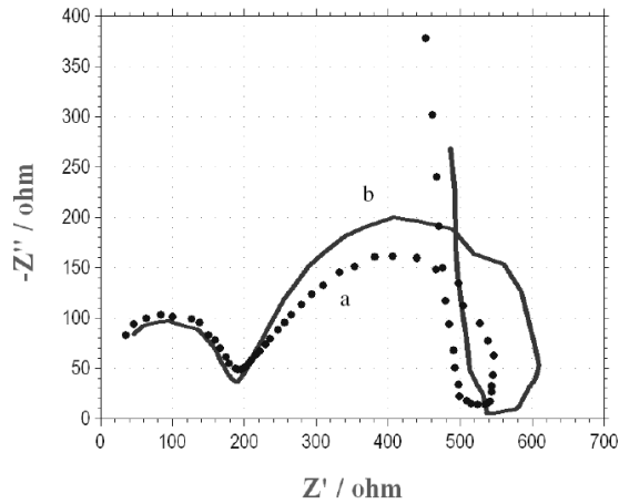
Figure 2 (a and b). AC impedance spectra of aluminium immersed in aqueous solution at pH 12 (NaOH). Nyquist plots: (a) aqueous solution at pH 12; (b) flower extract 8 mL + Zn^{2+} 50 ppm (pH 12).
