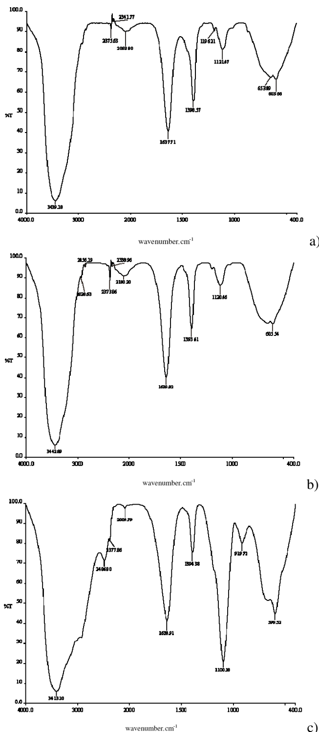
Figure 4. FTIR spectra (KBr). (a) Flower extract dried to solid mass; (b) Flower extract \text{Al}^{3+} complex; (c) Film formed on aluminium metal surface after immersion in the aqueous solution (pH 12) containing 8 mL of flower extract + 50 ppm of \text{Zn}^{2+} .
