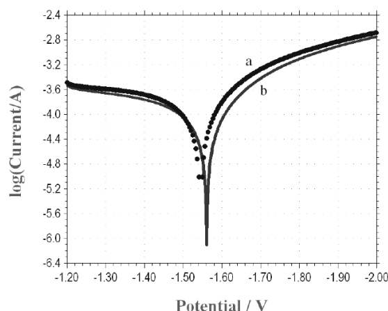
Figure 1. Polarization curves of aluminium immersed in aqueous solution at pH 12 (NaOH). (a) Aqueous solution at pH 12; (b) flower extract 8 mL + Zn 2+ 50 ppm (pH 12).
