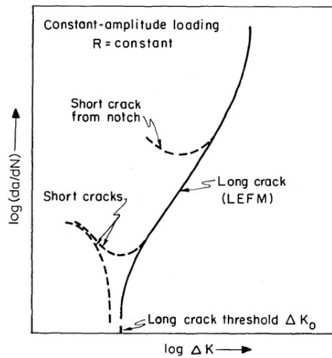
(a) Representation of small and long cracks growth in air [80].
