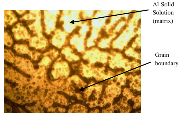
Figure 1: Micrograph of the as-cast Al-Cu-Ni alloy.
