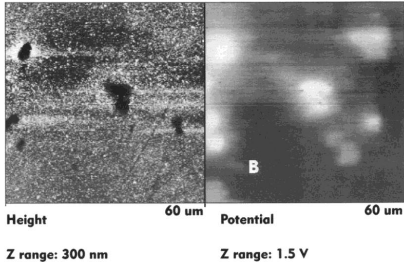
Fig. 4. Topography and Volta potential of the same area as Fig. 1 after 30 min of total exposure in 0.1 M NaCl.
