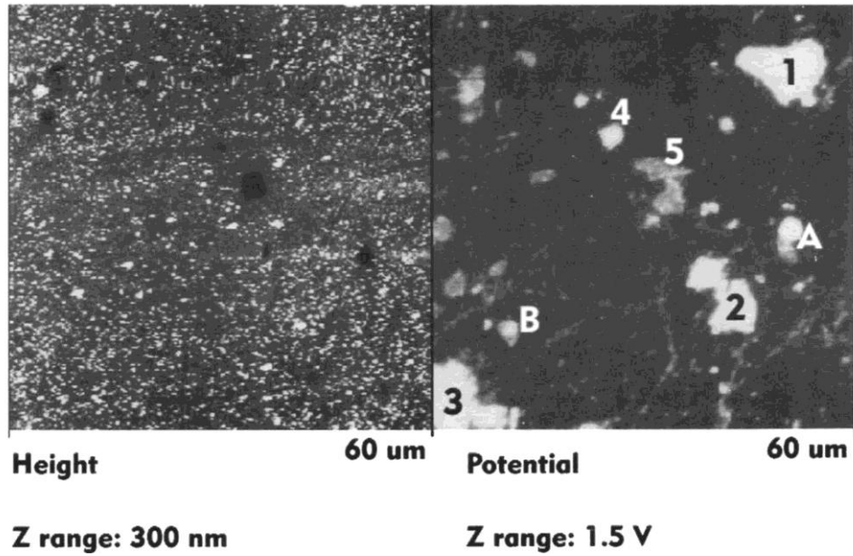
Fig. 1. Topography and Volta potential of an AA2024-T3 sample before treatment. Particles 1-5 are Al-Cu(Fe, Mn) intermetallics and particles A and B are the Al-Cu-Mg intermetallics.
