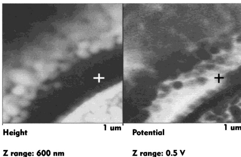
Fig. 11. Enlargement of Fig. 10 showing the trench formed around the particle. The marker indicates the bottom of the trench, which has a high potential.
