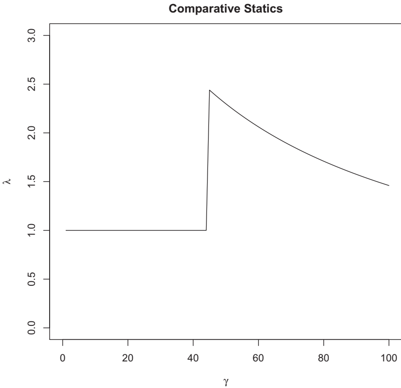
Figure 1. The Equilibrium Value of Anticorruption Commitments as a Function of Polarization. The equilibrium value of \lambda as a function of \gamma . Parameter values are fixed such that \alpha = 0.01 , \rho = 0.5 , and \kappa = 0.1 .
