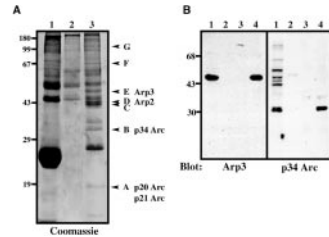
Figure 5. Association of the Arp2/3 complex with the cortactin amino terminus. (A) Identification of proteins interacting with the cortactin amino-terminal domain. Murine brain lysate was mixed with either GST-Sepharose (lane 1) or recombinant cortactin N-term-Sepharose
