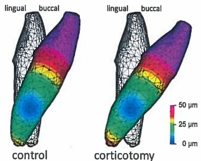
Figure 3. The total displacement of the lateral incisor in case of an uncontrolled tipping ( M/F = 0 ) for both the control and corticotomized models (with a deformed plot scaling factor of 100x). The centres of the dark areas correspond to the C_{rot} .
