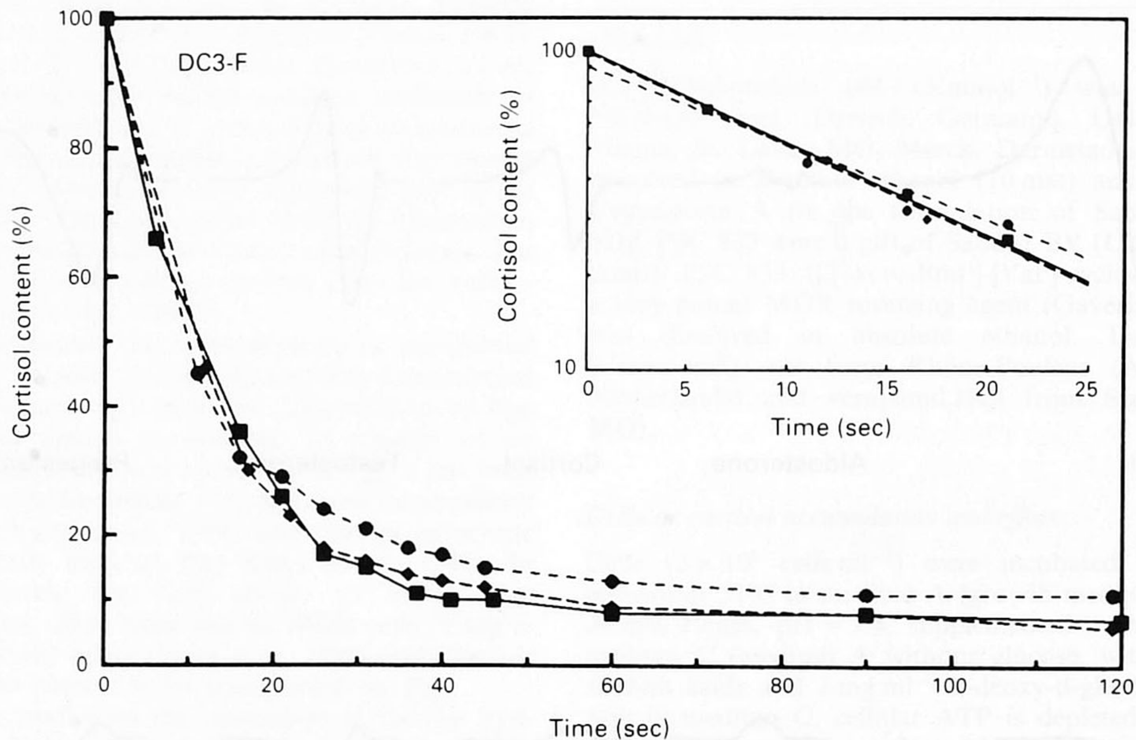
Figure 3 Efflux of cellular cortisol after loading DC3-F cells with 1 \mu\text{M} cortisol (set at 100%) and incubation in cortisol-free medium for the indicated times. Efflux in medium A ( \blacksquare — \blacksquare ), medium C ( \blacktriangle — \blacktriangle ) or medium A + 64 \mu\text{M} cyclosporin ( \blacklozenge — \blacklozenge ). Data are from a representative experiment; inset: linear regression curves. T_{1/2} values are in Table II.
