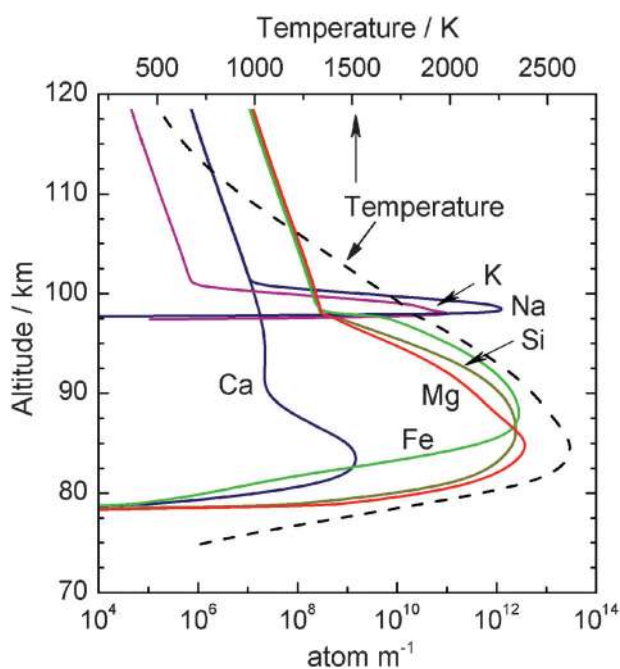
Fig. 3 Elemental ablation profiles for a 5 \mu\text{g} meteoroid entering at 20 \text{km s}^{-1} , as predicted by the Chemical Ablation Model (CABMOD). The particle temperature is shown on the top abscissa.
