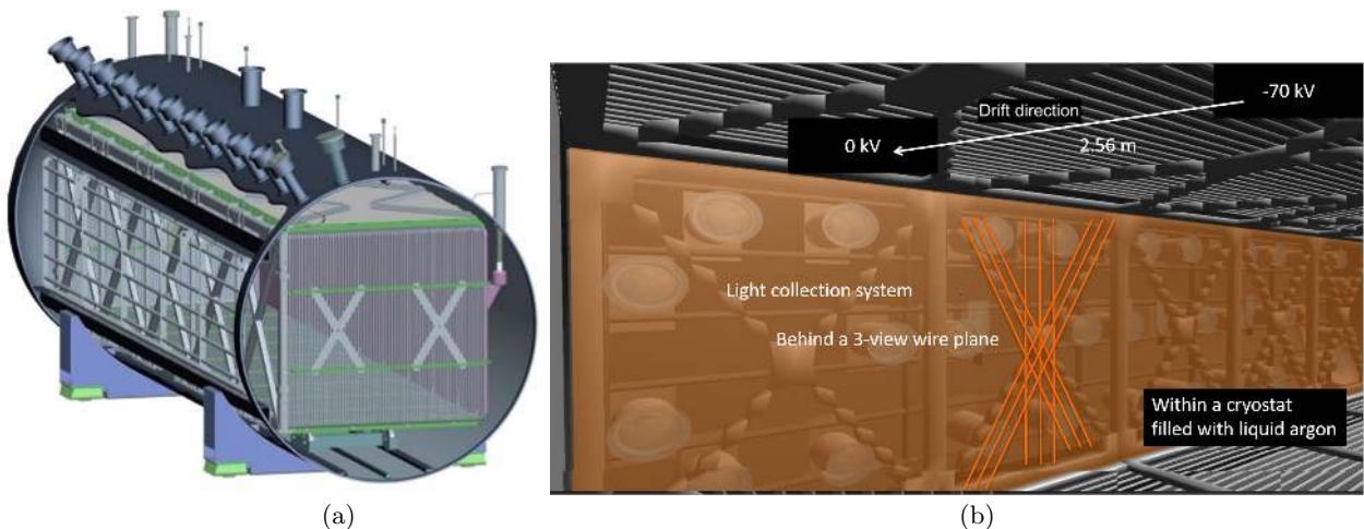
FIG. 2. (a) The MicroBooNE detector cryostat. The field cage is shown inside the cryostat. (b) Inside the cryostat of the MicroBooNE detector, visualized with the VENU software [32]. The maximum drift distance is 2.56 m with a drift electric field of 273 V/cm. The light-collection system, which consists of 32 PMTs, is located behind the three anode wire planes, which detect ionization charge.
