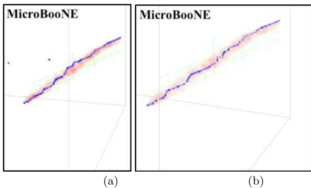
FIG. 25. Impact of adding charge information to the weight calculation. Blue points represent the shortest path. Space points are displayed in colors with their charge information. (a) Weights are calculated only according to distances. (b) Weights are calculated including the charge information.
