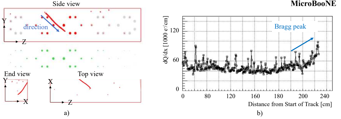
FIG. 6. Example of a stopped muon from MicroBooNE data.
