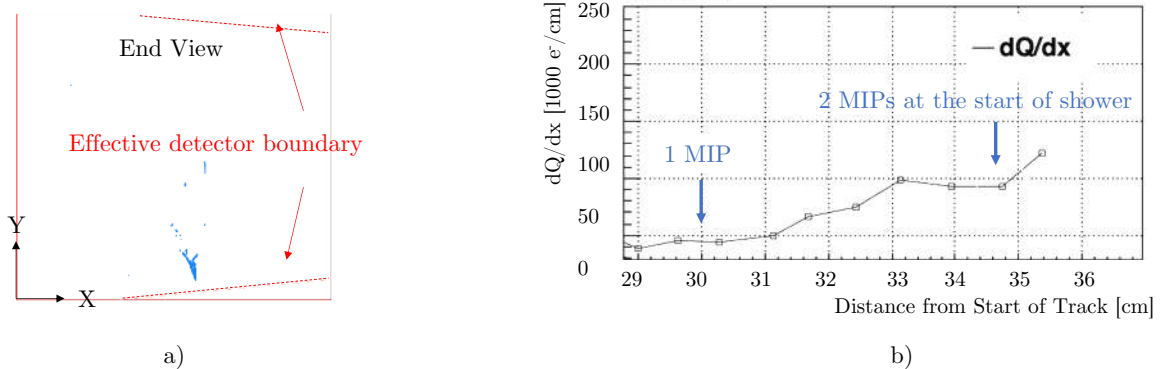
FIG. 9. Example of a gamma pair production from MicroBooNE data.
