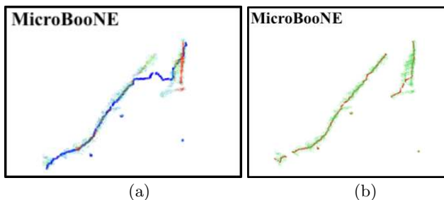
FIG. 19. (a) Track seed before applying the overclustering protection. As a result of the overclustering, track seed (blue points) is wrongfully constructed going through two separated clusters. Red and blue colors represent high and low charge, respectively. (b) Track seed after applying the overclustering protection. Two clusters (red points) are now properly separated. Space points are displayed as green points without charge information.
