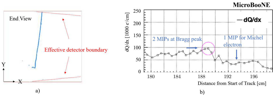
FIG. 13. A STM candidate with a short stopped muon track following by a Michel electron. A purple circle indicates the Bragg peak.
