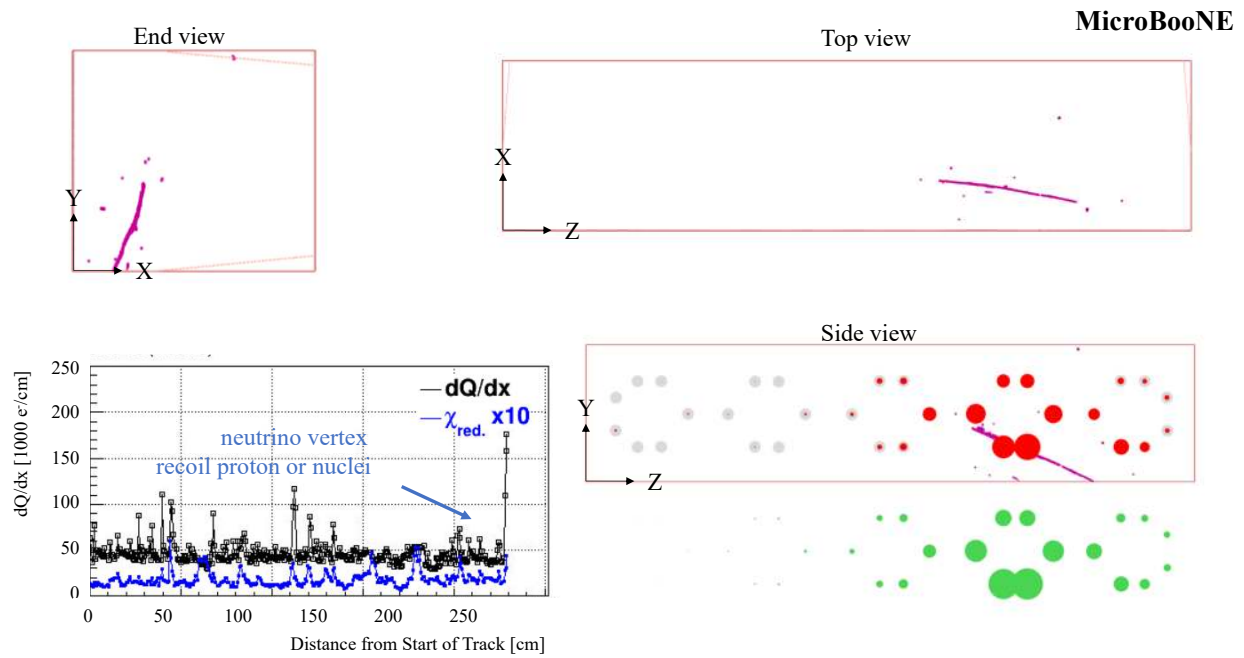
FIG. 30. A neutrino interaction candidate with a very large dQ/dx near the neutrino vertex. The sharp rise in dQ/dx (black line) near the end of track trajectory is presumably the result of a recoil proton or nucleus (see the plot of dQ/dx vs. Distance from start of track).
