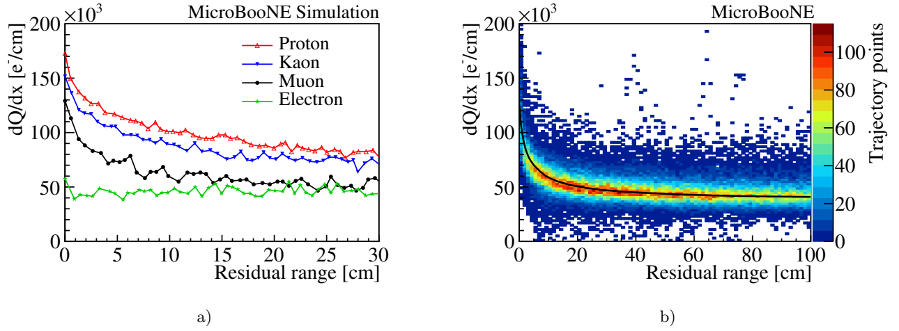
FIG. 7. (a) Examples of best-fit dQ/dx curves for different simulated stopped charged particles as a function of residual range (distance along the track with respect to the stopping location) using the fitting procedures described in this section. (b) The distribution of best-fit dQ/dx vs. residual range from a sample of \approx 2000 stopped muon tracks in MicroBooNE data. The color indicates number of trajectory points. The shape of the dQ/dx distribution is consistent with the model-predicted dQ/dx curve (black curve) of the muon. More details of this analytical model are described in Sec. V C.
