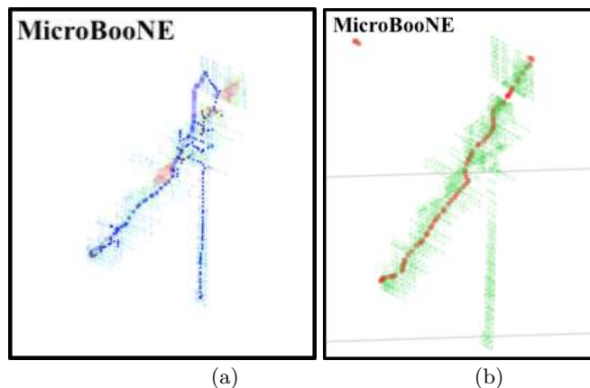
FIG. 24. Improvement in searching for end points. (a) Extreme points identification based on the principle component analysis. Space points are displayed in color with charge information. The shortest path is shown as blue points. (b) Current extreme points identification. Space points are displayed as green points without charge information. The shortest path is shown as red points.
