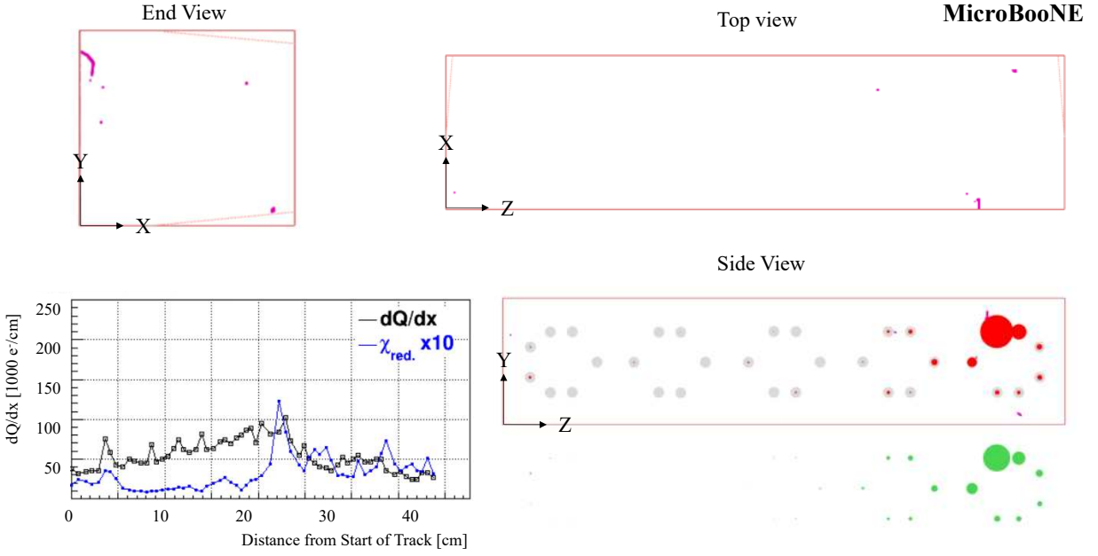
FIG. 28. A STM candidate with a short stopped muon track following by a Michel electron.
