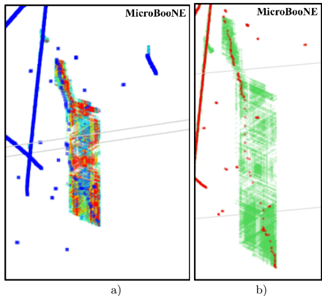
FIG. 23. Impact of the same-blob Steiner edges. (a) The shortest path (blue points) without adding the same-blob Steiner edges is along the boundary of the 3D image. This is partially caused by the grid structure of space points. Space points without charge information are displayed as green. (b) The shortest path after adding the same-blob Steiner edges (red points). Space points are displayed as green without the charge information.
