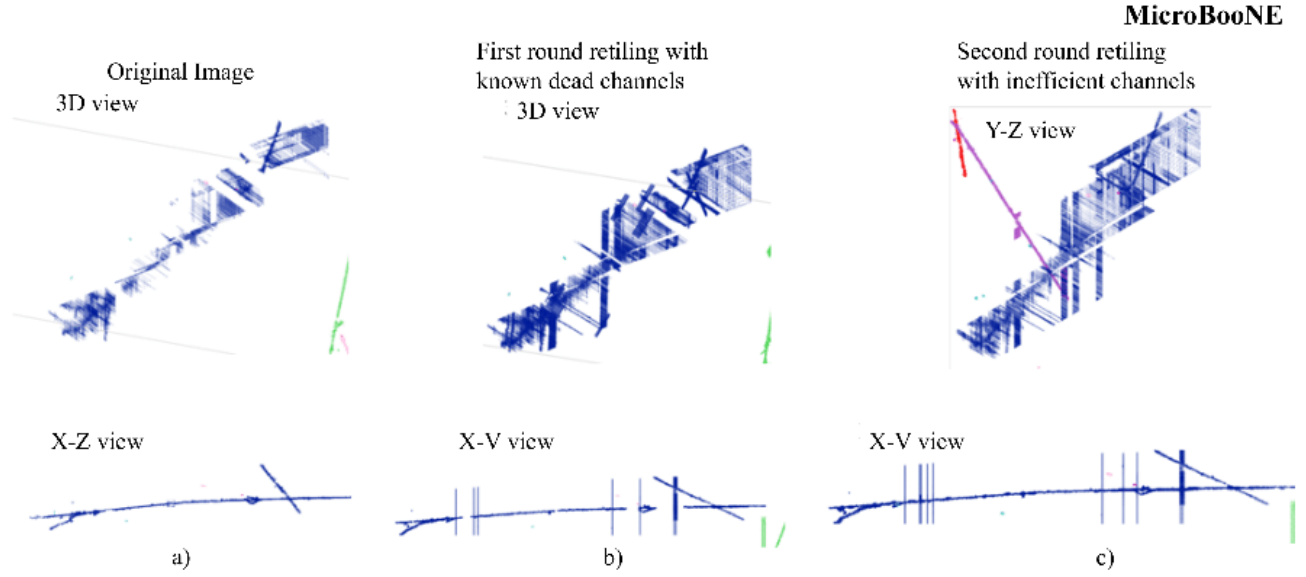
FIG. 20. Illustration of the retiling step. (a) Original images are shown for 3D (top) and X-Z projection (bottom) views. (b) The same images for 3D (top) and X-V projection (bottom) after the first round of retiling when the known nonfunctional channels are filled. (c) Same images for Y-Z projection (top) and X-V projection (bottom) after the second round of retiling, which fills the inefficient channels.
