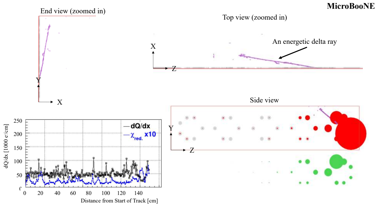
FIG. 31. A neutrino interaction candidate with an energetic delta ray. The track direction is obvious after taking into account the direction of the energetic delta ray. There is a rise in dQ/dx near the stopping point tagged by the STM evaluation algorithm described in Sec. V C. This rise is partially because of the dip in dQ/dx in the region just before the stopping point.
