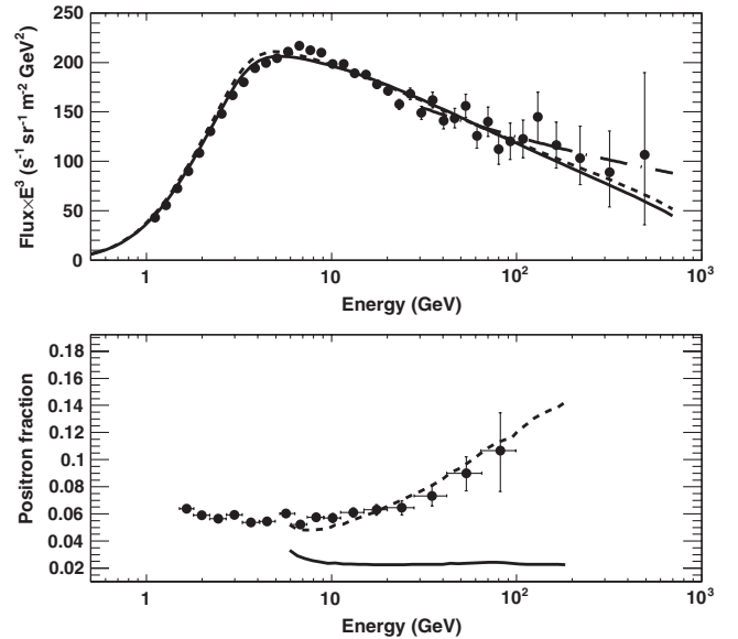
FIG. 3. Top: the e^- spectrum obtained in this work compared with theoretical calculations. The solid line shows the standard GALPROP calculation [29] for a diffusion reacceleration model; the long-dashed line is a single power-law fit to the data above 30 GeV; the short-dashed line is a GALPROP calculation including a component from additional cosmic-ray electron sources. Bottom: the PAMELA positron fraction [28] compared with the previous GALPROP calculations with no (solid line) and with additional e^- and e^+ components (short-dashed line). The error bars are statistical only and these were the only errors considered by the fitting procedures.
