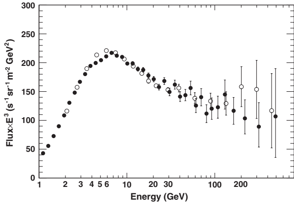
FIG. 1. The negatively charged electron spectrum measured by PAMELA with two independent approaches: energy derived from the rigidity (full circles); energy derived from the calorimeter information (open circles). The error bars are statistical only.
