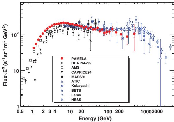
FIG. 2 (color). The electron energy spectrum obtained in this work compared with modern measurements: CAPRICE94 [19], HEAT [20], AMS [21], MASS91 [22], Kobayashi [23], BETS [24], ATIC [25], HESS [26], Fermi [27]. Note that the data points from [23–27], indicated with blue symbols, and the highest data point from HEAT [20] are for the electron and positron sum.
