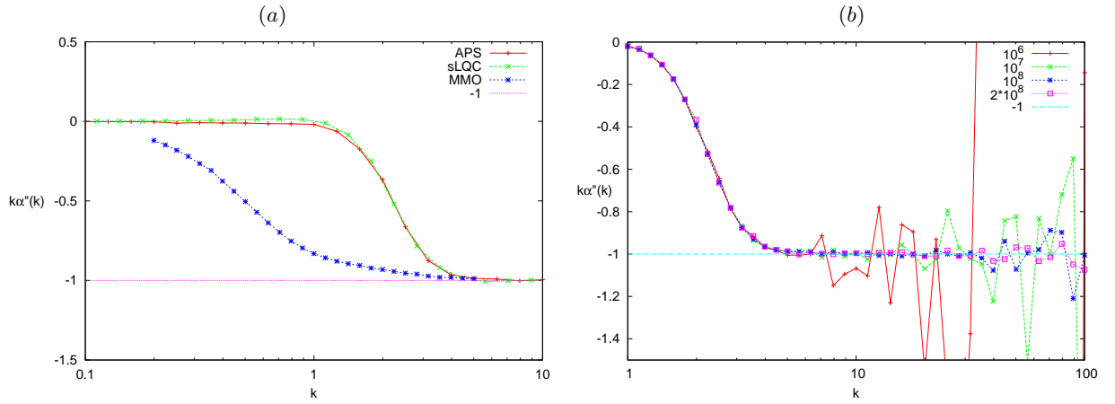
FIG. 3: (a) The rescaled derivative k\partial_k^2 \alpha for different quantization prescriptions shown in the domain, where it could be determined numerically in the reliable manner. (b) The values of k\partial_k^2 \alpha for APS prescription evaluated on different sets of probing points with the upper bound ranging from 10^7 to 2 \cdot 10^8 . The numerical solutions converge as the bound increases.
