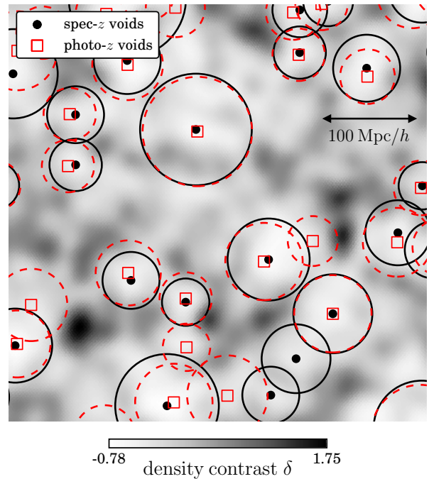
Figure 4. Comparison between voids found in spec-z (centers: solid black points; radius: solid black circles) and photo-z (centers: open red squares; radius: red dashed circles) in the simulations for a slice of thickness 2s_v = 100 Mpc/h. The background gray-scaled field is the smoothed galaxy field ( \sigma = 10 Mpc/h) used by the void-finder. The correlation between spec-z and photo-z defined voids is clear: in many cases the void position and radius match almost exactly.
