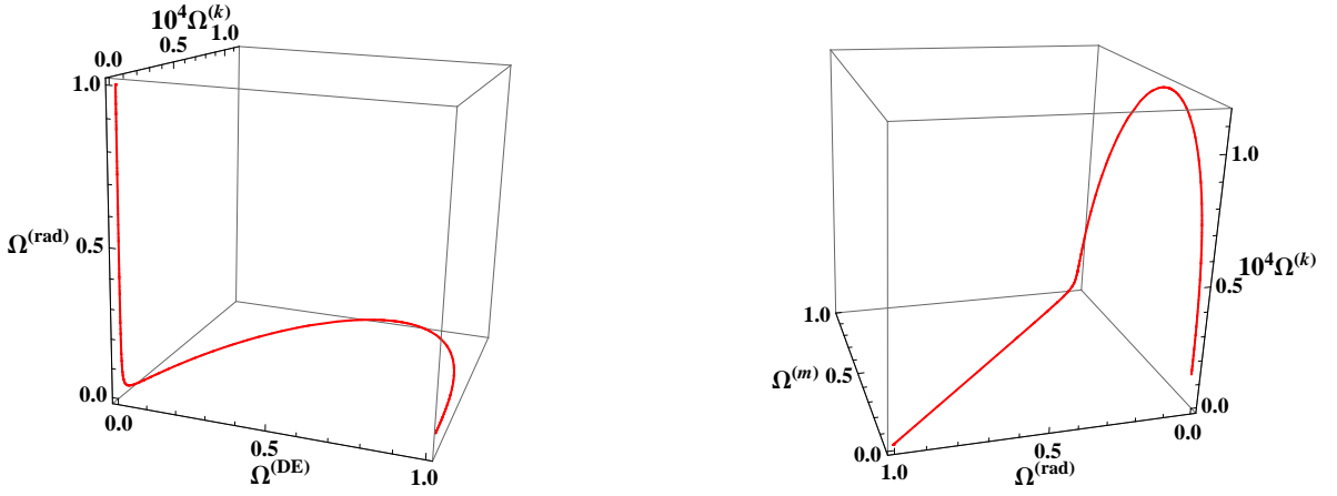
Figure 7. (color online). Cosmological solutions of f(R, T) = R + c_1 \sqrt{-T} gravity for k = -1 . The left parametric plot is in terms of \Omega^{(k)} , \Omega^{(\text{rad})} , and \Omega^{(\text{DE})} , and the right one is in terms of \Omega^{(k)} , \Omega^{(\text{rad})} , and \Omega^{(\text{m})} coordinates. The peaks of the curves occur at \Omega^{(\text{DE})} \simeq 0.7 in the left and at \Omega^{(\text{m})} \simeq 0.3 in the right diagrams, respectively.
