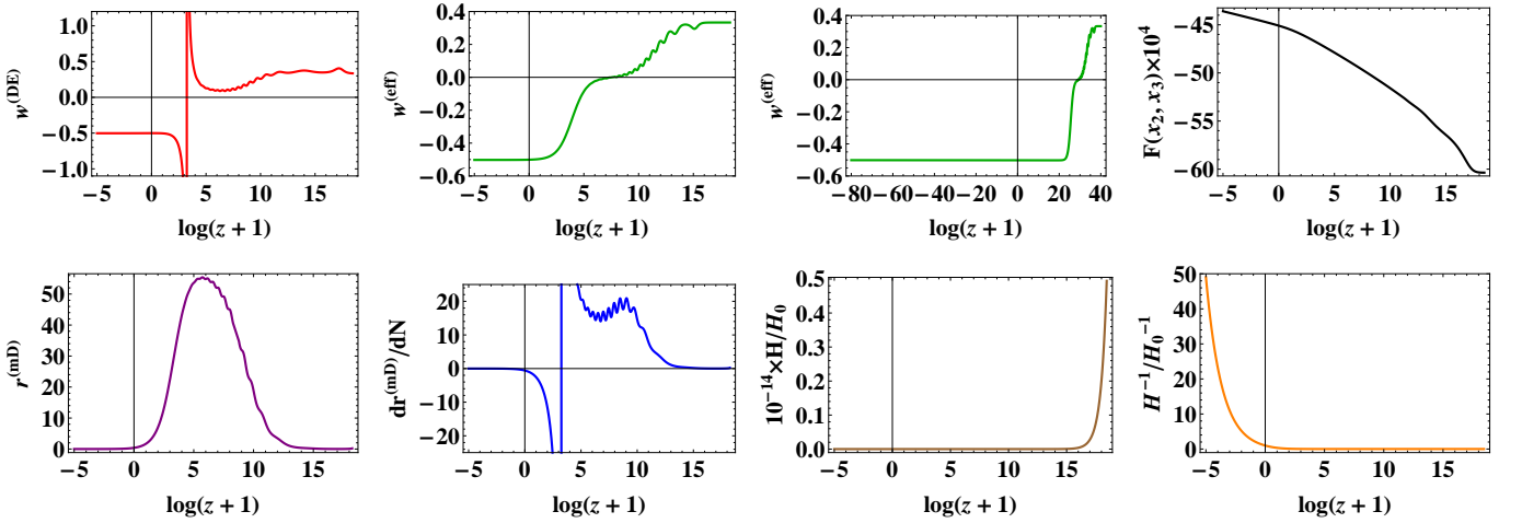
Figure 2. (color online). Cosmological solutions of f(R, T) = R / \log(\alpha R) + \sqrt{-T} gravity. The initial values are x_1 = 10^{-9} , x_2 = -10^{-3} , x_3 = 1.006 \times 10^{-3} , x_4 = 2.3 \times 10^{-16} and x_5 = 0.9999 corresponding to z \approx 1.03 \times 10^8 . We used \alpha = 5.7 \times 10^{61} in some plots. The numerical data are matched to the present values of \Omega_0^{(m)} \approx 0.3 , \Omega_0^{(rad)} \approx 10^{-4} and H_0 \simeq 67.3 km/(Mpc.s) . In this case, the values of F(x_2, x_3) are negative, which is not accepted. The matter-dominated era happens in the redshift z \sim 60 , and the relative size of the universe in this era is about 4.1 \times 10^{-3} .
