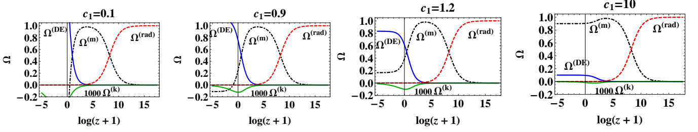
Figure 5. (color online). The effects of coupling constant c_1 on the fluid density parameters in f(R, T) = R + c_1\sqrt{-T} gravity for an open universe. The radiation density parameter is not affected by this constant. The larger (smaller) values of c_1 leads to small (larger) values of the dark energy and the spatial curvature densities.
