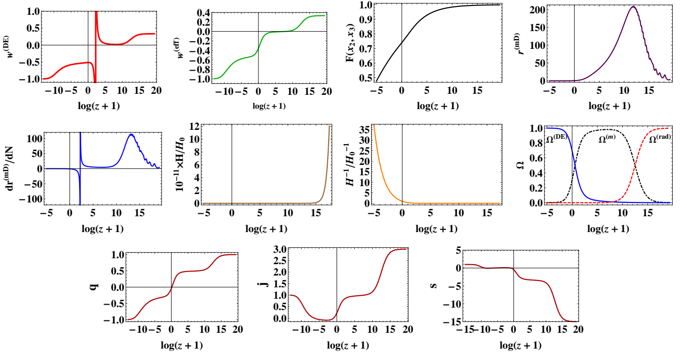
Figure 4. (color online). Cosmological solutions of f(R, T) = R + \alpha R^{0.9} + \sqrt{-T} gravity. For this theory, we have chosen the initial values x_1 = 10^{-6} , x_2 = -10^{-3} , x_3 = 1.0001 \times 10^{-3} , x_4 = 0.45 \times 10^{-15} , and x_5 = 0.999 that correspond to z \approx 2.6 \times 10^8 with \alpha = 4.06 \times 10^{-5} . The initial values are chosen in a way that the matter era occurs in the redshift of about z_m \simeq 1100 , which corresponds to the last scattering surface. With these initial values, the radiation–matter equality takes place at z \simeq 10^5 , which is far from the given results in the literature. Note that it is possible to choose some other initial values to solve this inconsistency, however, one should be careful about the other cosmological quantities, such as the value of the function F . The above diagrams for the deceleration, jerk, and snap parameters show a consistent sequence for different cosmological eras. However, their present values do not match the present observational data. For this theory, the relative size of the universe in this era is about 1.2 \times 10^{-5} .
