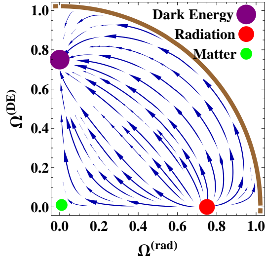
Figure 8. (color online). A phase portrait for the special case k = 0 is drawn. There is an acceptable trajectory that connects the radiation era to the matter era then to the dark-energy-dominated era as the final attractor. The other trajectories do not contain any proper cosmological sequence.
