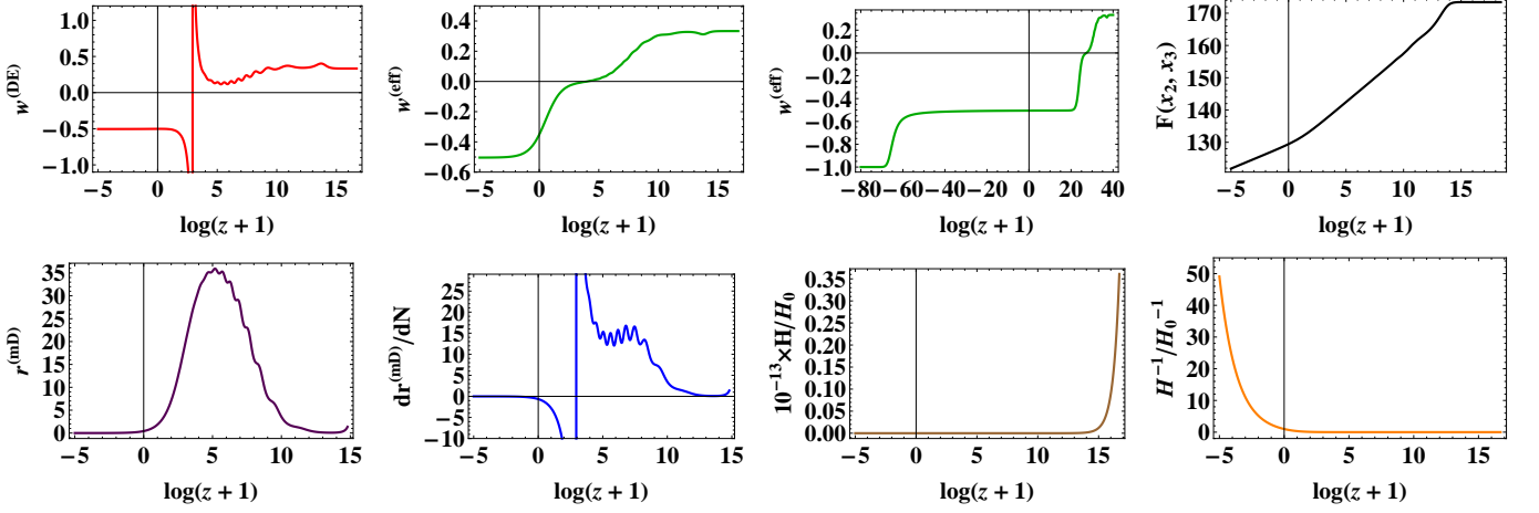
Figure 1. (color online). Cosmological solutions of f(R, T) = R \log(\alpha R) + \sqrt{-T} gravity. The different cosmological parameters consist of the dark energy equation of state, the effective equation of state, F(x_2, x_3) , the ratio of the matter density to the dark energy density and its first derivative, and the Hubble parameter and its inverse. The initial values x_1 = 10^{-7} , x_2 = -10^{-6} , x_3 = 1.0058 \times 10^{-6} , x_4 = 0.3 \times 10^{-14} , and x_5 = 0.9999 correspond to z \approx 1.78 \times 10^7 . We used \alpha = 1.95 \times 10^{92} in some plots. The diagrams are drawn to be consistent with the present value of \Omega_0^{(m)} \approx 0.3 , \Omega_0^{(rad)} \approx 10^{-4} and H_0 \simeq 67.3 km/(Mpc.s) . As it is obvious, the diagram for F(x_2, x_3) has not a suitable range of value to indicate a matter-dominated era for which F \approx 1 . The diagram of r^{(mD)} shows that the value of 3/7 appears twice in the evolution of the cosmos, and its ratio is about -0.6 at the present era. The matter dominates in the redshift z \sim 33 , and from the diagram for H^{-1} , we find that in this epoch the relative size of the universe is about 9.4 \times 10^{-3} .
