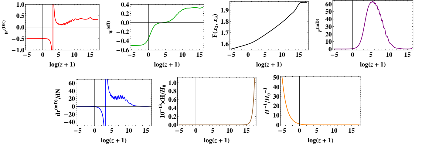
Figure 3. (color online). Cosmological solutions of f(R, T) = R + \alpha R^{1.01} + \sqrt{-T} gravity. In this case, the initial values x_1 = 10^{-8} , x_2 = -10^{-5} , x_3 = 1.0049 \times 10^{-5} , x_4 = 10^{-15} , and x_5 = 0.9999 correspond to z \approx 3.6 \times 10^7 . We have used \alpha = 1.43 in some plots. In this theory, we reach at the same results as the previous two theories in subsection III A, except the result of the function F , which is more reasonable in this theory. The matter-dominated era for the theory with n = -1.01 occurs in z \sim 43 with the relative size of the universe in this era about 6 \times 10^{-3} .
