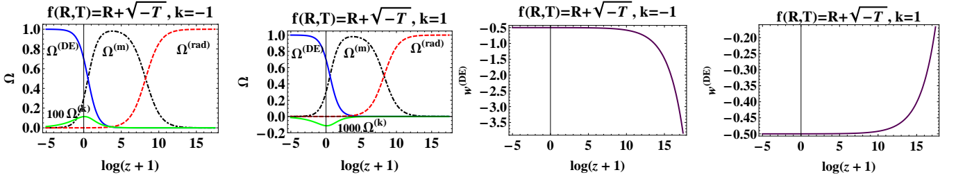
Figure 6. (color online). Cosmological solutions of f(R, T) = R + c_1\sqrt{-T} gravity with c_1 = 1 . These diagrams accept the initial values \Omega^{(\text{rad})} = 0.9999 , \Omega^{(\text{DE})} = 10^{-15} , and \Omega^{(k)} = 10^{-15} for an open universe and the same values, but with \Omega^{(k)} = -10^{-15} , for a closed universe, corresponding to z \approx 3.6 \times 10^7 . The diagrams show \Omega_0^{(k)} = 10^{-3} for the open universe and \Omega_0^{(k)} = -10^{-4} for the closed universe. The dark energy curve has an increasing behavior up to the value w^{(\text{eff})} = -1/2 for the open universe, and it has a decreasing behavior down to the value w^{(\text{eff})} = -1/2 for the closed universe.
