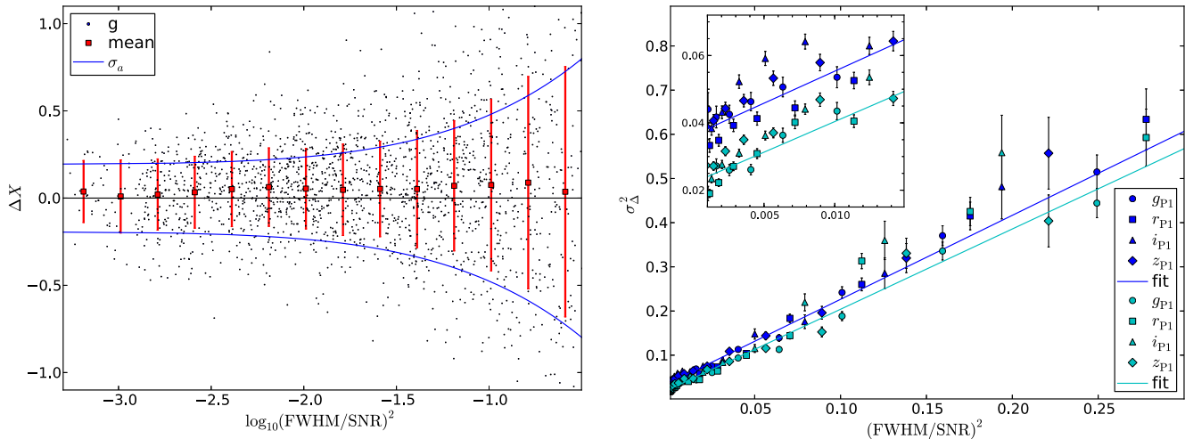
Figure 17. Left panel: the position difference \Delta X in pixels of nightly and deep stacks for stars from 100 randomly selected g_{P1} band images (black dots) vs. \log_{10}(\text{FWHM}/(\text{S}/\text{N}))^2 . The red circles and its error bars indicate the average \Delta X in appropriate (\text{FWHM}/(\text{S}/\text{N}))^2 bins and its standard deviation \sigma_{\Delta X} , respectively. The blue line is the fitted \sigma_{\Delta X} from the fit shown in the right panel. Right panel: the measured variance \sigma_{\Delta X}^2 and \sigma_{\Delta Y}^2 in blue and cyan symbols, respectively, for all four bands vs. (\text{FWHM}/(\text{S}/\text{N}))^2 . The straight line fits are shown with the solid lines. The inset shows that for very small (\text{FWHM}/(\text{S}/\text{N}))^2 , there is a significant difference in X and Y direction.
