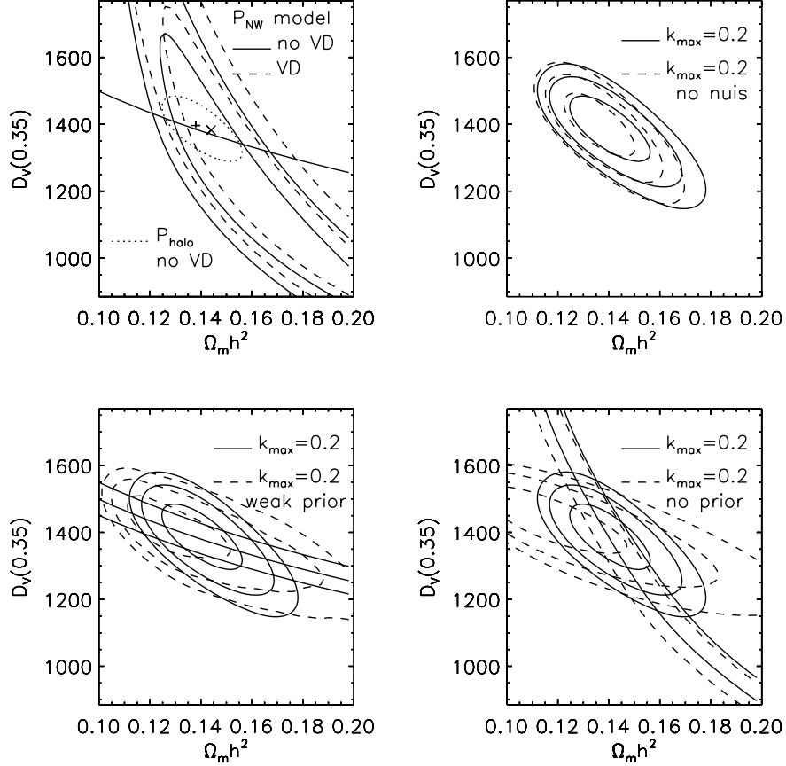
Figure C1. Effects of velocity dispersion and nuisance parameters on constraints from the LRG DR7 \hat{P}_{\text{halo}}(k) for a \Lambda CDM model. In each panel, we hold \Omega_b h^2 = 0.02265 and n_s = 0.960 fixed. Upper left-hand panel: \Delta\chi^2 = 2.3 and 6.0 contours for the \hat{P}_{\text{halo}}(k) fit to a no-wiggles model with no central velocity dispersion (solid) and extreme velocity dispersion (dashed). The \Delta\chi^2 = 2.3 for the fiducial model with BAO features is shown for comparison by the dotted line. The cross shows the maximum likelihood point for our fiducial model, while the ‘X’ shows it for the extreme velocity dispersion model. The solid line indicates r_s/D_V(0.35) = 0.1097 , demonstrating that adopting the velocity dispersion model shifts the likelihood surface along constant r_s/D_V(0.35) . Upper right-hand panel: \Delta\chi^2 = 2.3 , 6.0 and 9.3 contours. The solid contours use our fiducial marginalization over b_0^2 , a_1 and a_2 (as in Fig. 5), while in the dotted contours fix a_1 = a_2 = 0 and b_0^2 to the value which minimizes \chi^2 . Lower left-hand panel: the solid contours as in Fig. 5, while the dashed contours take the minimum \chi^2 value for which |F(k = 0.1 \text{ h Mpc}^{-1})|/b_0^2 < 0.2 and |F(k = 0.2 \text{ h Mpc}^{-1})|/b_0^2 < 0.5 . Lower right-hand panel: the solid contours as in Fig. 5, while the dashed contours minimize \chi^2 with no restrictions on a_1 and a_2 . For comparison with the fiducial nuisance restrictions, the solid lines enclose the region where for the best-fitting \chi^2 , |F(k = 0.1 \text{ h Mpc}^{-1})|/b_0^2 < 0.04 and the dashed lines enclose |F(k = 0.2 \text{ h Mpc}^{-1})|/b_0^2 < 0.1 .
