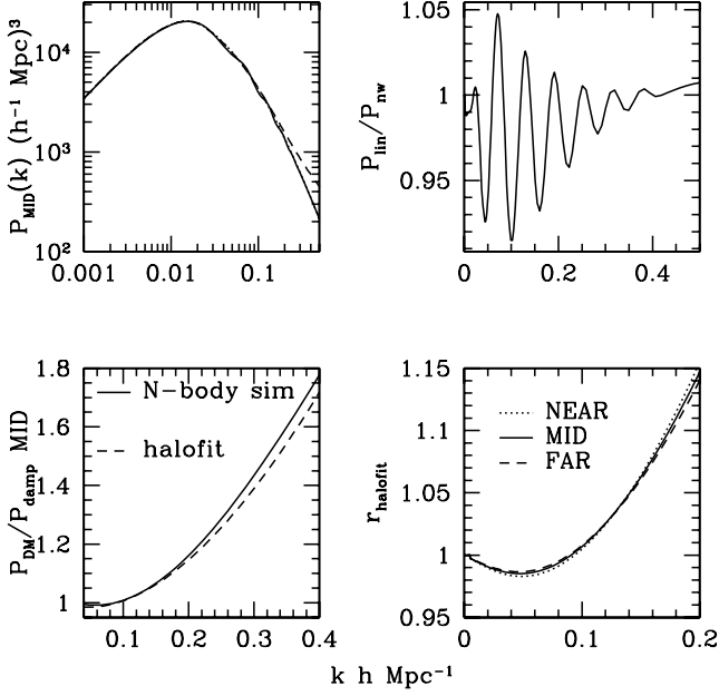
Figure 3. Upper left-hand panel: power spectra for the fiducial cosmology. The solid curve is P_{lin}(k) and the dashed curve is P_{nw}(k)r_{haloFIT} , the non-linear power spectrum from HALOFIT using P_{nw}(k) as the input. Upper right-hand panel: P_{lin}(k)/P_{nw}(k) . Lower left-hand panel: P_{DM}(k)/P_{damp}(k, \sigma_{DM}) measured in N -body simulation snapshots at z_{MID} , reported in Reid et al. (2009), compared with the smooth correction predicted by HALOFIT, r_{haloFIT} . Lower right-hand panel: r_{haloFIT} at \{z_{NEAR}, z_{MID}, z_{FAR}\} = \{0.235, 0.342, 0.421\} .
