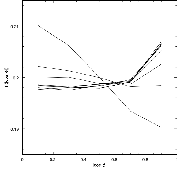
Figure A1. P(|\cos \phi|) versus \cos \phi where \phi is the angle between the galaxy pair separation vector and the line of sight defined by the observer and one of the galaxies in the pair (see text). The smallest separation bin ( 15 h^{-1} Mpc < \Delta r < 30 h^{-1} Mpc) shows the largest deviation from isotropy, with an \sim 5 per cent preference for pairs perpendicular to the line of sight compared to along the line of sight due to FOGs. The larger separation bins extend to 150 h^{-1} Mpc and are nearly isotropic, but with a few per cent excess of pairs directly along the line of sight.
