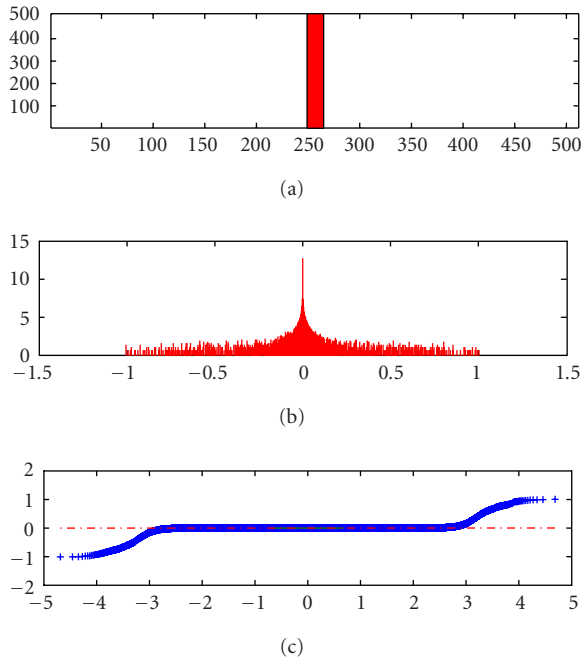
FIGURE 10: (a) The image of the bar, (b) the log-histogram of the curvelet coefficients of the bar, and (c) the qq-plot of the curvelet coefficients versus normal distribution.
