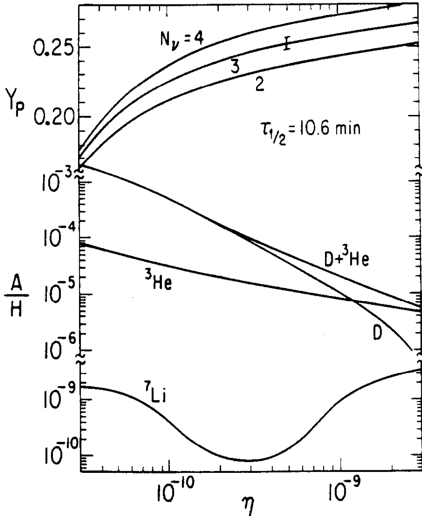
Fig. 1.2 The predicted primordial abundances of D, {}^3\text{He} , {}^4\text{He} , and {}^7\text{Li} . [Note \tau_{1/2} = 10.6 \text{ min} was used; error bar shows \Delta\tau_{1/2} = \pm 0.2 \text{ min} ; Y_p = mass of {}^4\text{He} ; N_\nu = equivalent number of light neutrino species.] Inferred primordial abundances: Y = 0.23\text{--}0.25 ; (\text{D}/\text{H}) > 1 \times 10^{-5} ; (\text{D} + {}^3\text{He})/\text{H} < 10^{-6} ; {}^7\text{Li}/\text{H} = (1.1 \pm 0.4) \times 10^{-10} . Concordance requires: \eta = (4\text{--}7) \times 10^{-10} and N_\nu \leq 4 .
