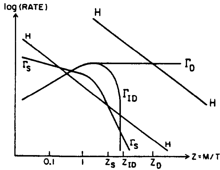
Fig. 2.2 Important rates as a function of z = M/T . H is the expansion rate, \Gamma_D the decay rate, \Gamma_{ID} the inverse decay rate, and \Gamma_S the 2^D \leftrightarrow 2^B scattering rate. Upper line marked H corresponds to case where K \ll 1 ; lower line the case where K > 1 . For K \ll 1 , X s decay when z = z_D ; for K > 1 , freeze out of ID s and S occur at z = z_{ID} and z_S .
