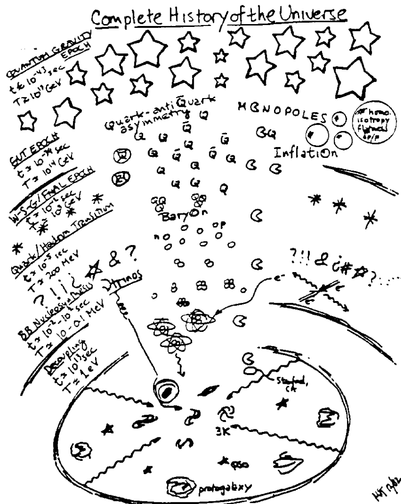
Fig. 1.1 'The Complete History of the Universe'. Highlights include: decoupling ( t = 10^{11} s, T = 1/3 eV) - the surface of last scattering for the cosmic microwave background, epoch after which matter and radiation cease to interact and matter 'recombines' into neutral atoms ( D , {}^3\text{He} , {}^4\text{He} , {}^7\text{Li} ); also marks the beginning of the formation of structure; primordial nucleosynthesis ( t = 10^2 s, T = 10 MeV) - epoch during which all of the free neutrons and some of the free protons are synthesized into D , {}^3\text{He} , {}^4\text{He} , and {}^7\text{Li} , and the surface of last scattering for the cosmic neutrino backgrounds; quark/hadron transition ( t = 10^{-5} s, T = \text{few } 100 MeV) - epoch of 'quark enslavement' [confinement transition in SU(3) ]; W-S-G epoch associated with electroweak breaking, SU(2) \times U(1) \rightarrow U(1) ; GUT epoch (?? t = 10^{-36} s, T = 10^{16} GeV??) - SSB of the GUT, during which the baryon asymmetry of the Universe evolves, monopoles are produced, and 'inflation' may occur; the Quantum Gravity Wall ( t = 10^{-43} s, T = 10^{19} GeV).
