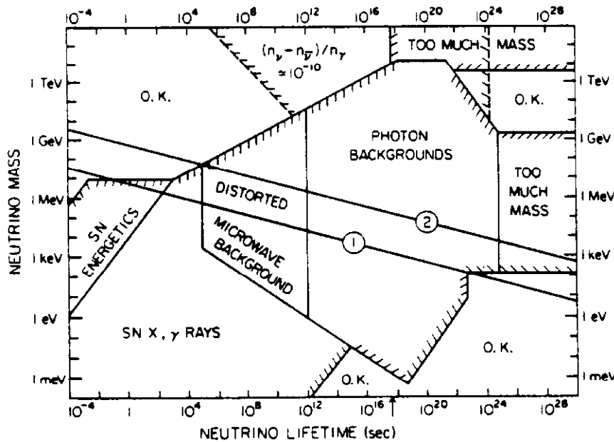
Fig. 1.6 Summary of astrophysical/cosmological constraints on neutrino masses/lifetimes. Lines 1 and 2 represent mass/lifetime relationships: \tau = a \times 10^{-6} \text{ sec } (m_{\nu} / m_{\mu})^5 , for a = 1, 10^{12} .
