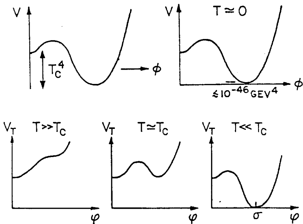
Fig. 4.2 The finite temperature effective potential V_T , for T > T_c ; T = T_c ; and T < T_c ; here \phi = \sigma is the SSB minimum of V_c .
