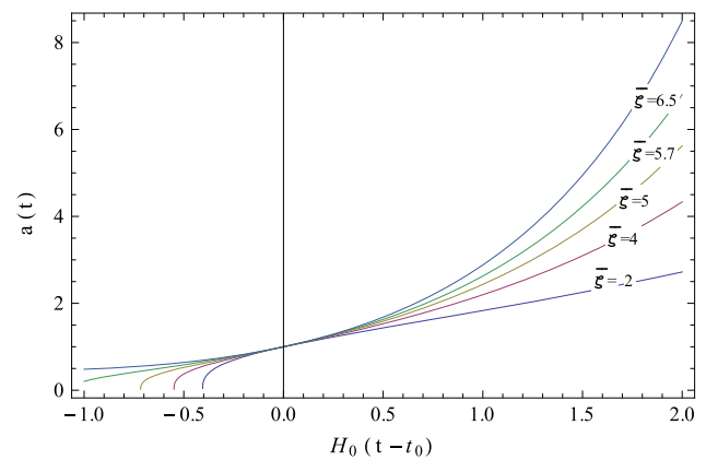
Fig. 2 Evolution of the scale factor a(t) with H_0(t - t_0) for different values of dimensionless bulk viscous parameter \bar{\zeta}
