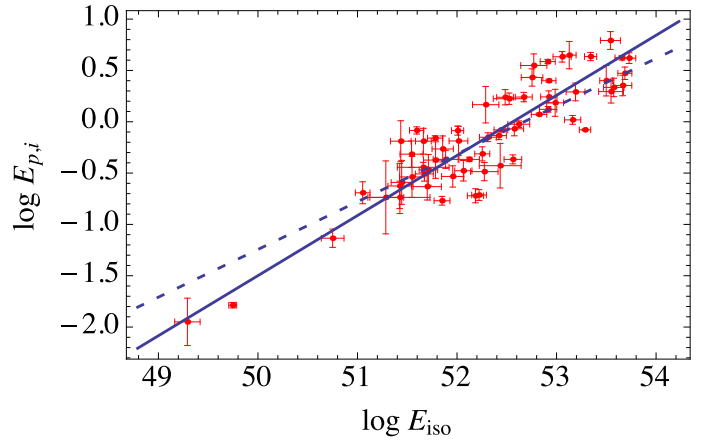
Fig. 5. Best-fit curves for the E_{\text{iso}}-E_{p,i} correlation relation superimposed on the data. The solid and dashed lines refer to the results obtained with the maximum likelihood (Reichart likelihood) and weighted \chi^2 estimator, respectively.
