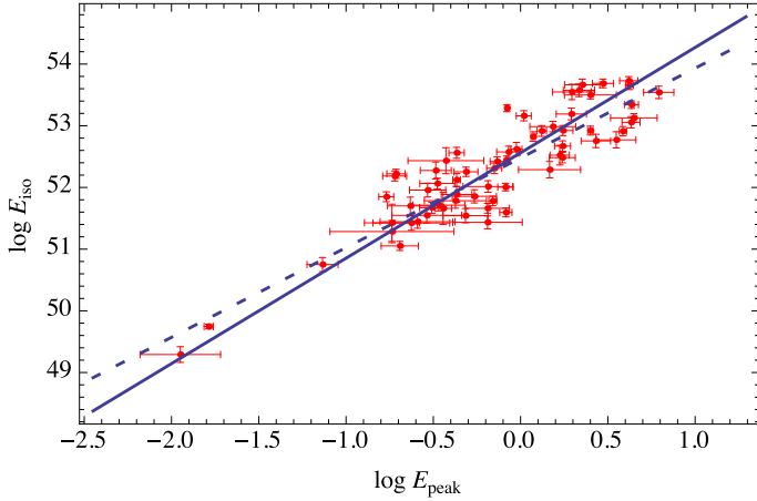
Fig. 3. Best-fit curves for the E_{p,i}-E_{\text{iso}} correlation relation superimposed on the data. The solid and dashed lines refer to the results obtained with the maximum likelihood (Reichart likelihood) and weighted \chi^2 estimator, respectively.
