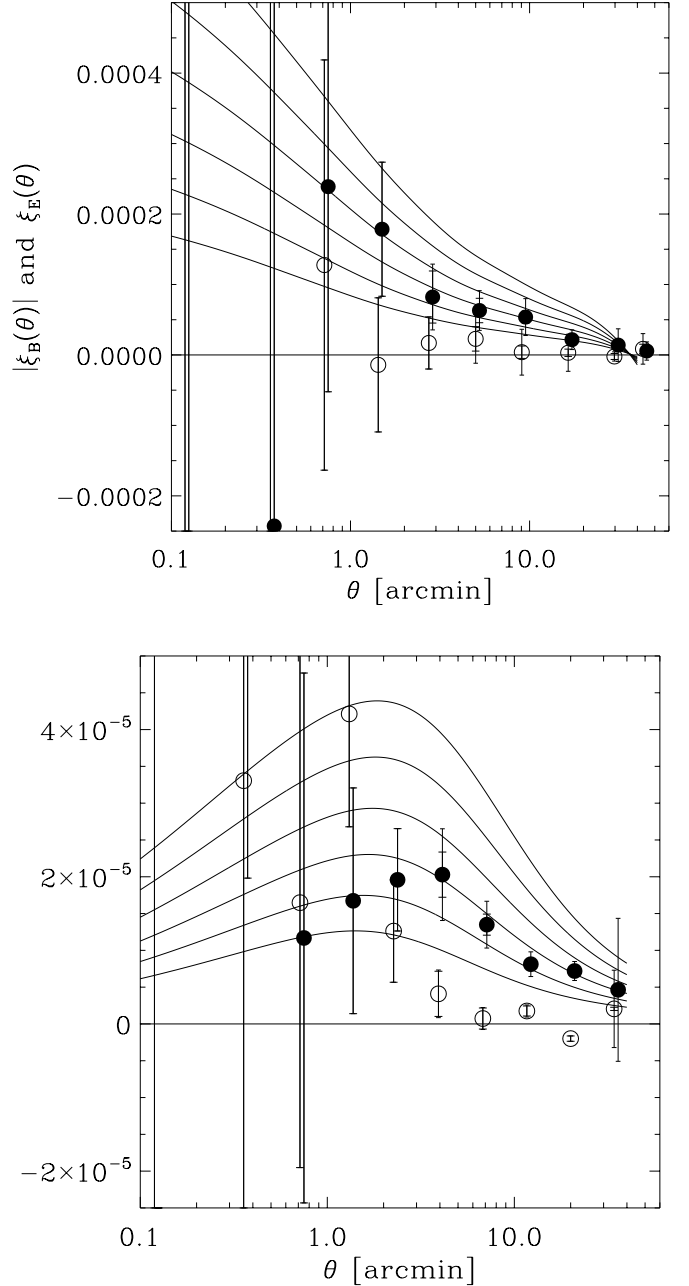
FIG. 6.— E - B decompositions of the 2D shear field. The top panel shows the statistics that formally require an integral over the measured correlation functions to infinite scales, and the bottom panel shows those that formally require an integral from zero. Filled circles show the E -mode, and open circles show the B -mode. The lines show predictions in a concordance cosmology with \sigma_8 varying as in Fig. 2. Note that adjacent data points in the top panel are highly correlated.
