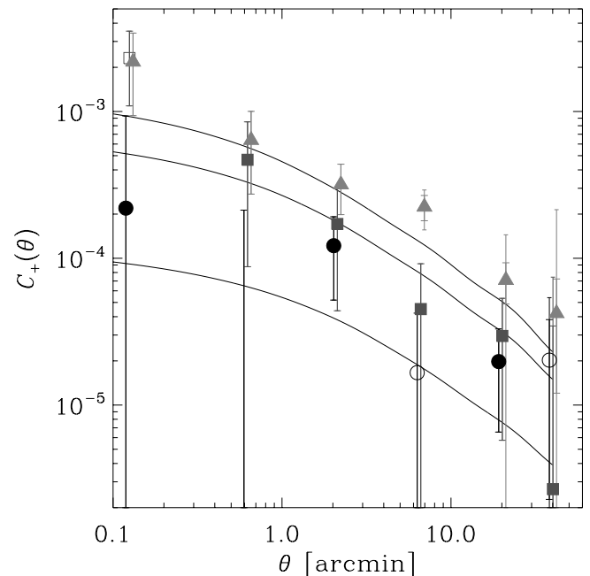
FIG. 8.— Evolution of the cosmic shear two-point correlation function signal with increasing redshift. The series of data points, (circles, squares, then triangles), show measurements from slices between redshifts 0.1, 1, 1.4, and 3. The black curves show predictions from a flat \Lambda CDM model with \Omega_m = 0.3 and \sigma_8 = 0.85 , for the same slices, increasing in redshift from the bottom to the top. Open circles depict negative values. [See the electronic edition of the Supplement for a color version of this figure.]
