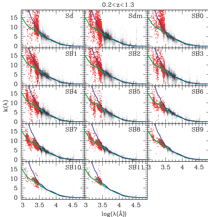
Figure 4. Attenuation by dust as a function of \lambda . The points are the extinction A_i/(E_i(B - V)) estimated from the galaxies with a spectro- z (see Section 3.4). The red points at \lambda < 3000 \text{ \AA} are not used to estimate E_i(B - V) . The Prevot et al. (1984) and Calzetti et al. (2000) extinction curves are shown with the blue and green solid lines, respectively. The Prevot et al. (1984) extinction law is rescaled to the same A_V as the Calzetti law by applying a factor of 4.05/2.72 . The extinction curve derived by Prevot et al. (1984) is used for the galaxies redder than SB3 and the Calzetti et al. (2000) extinction law for the galaxies bluer than SB3.
