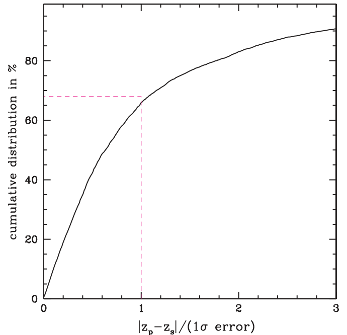
Figure 8. Cumulative distribution of the ratio |z_p - z_s| / (1\sigma \text{ error}) . Sixty-five percent of the photo-z have a spectro-z solution encompassed within the 1\sigma error, close to the expected value of 68% (magenta dashed line).
