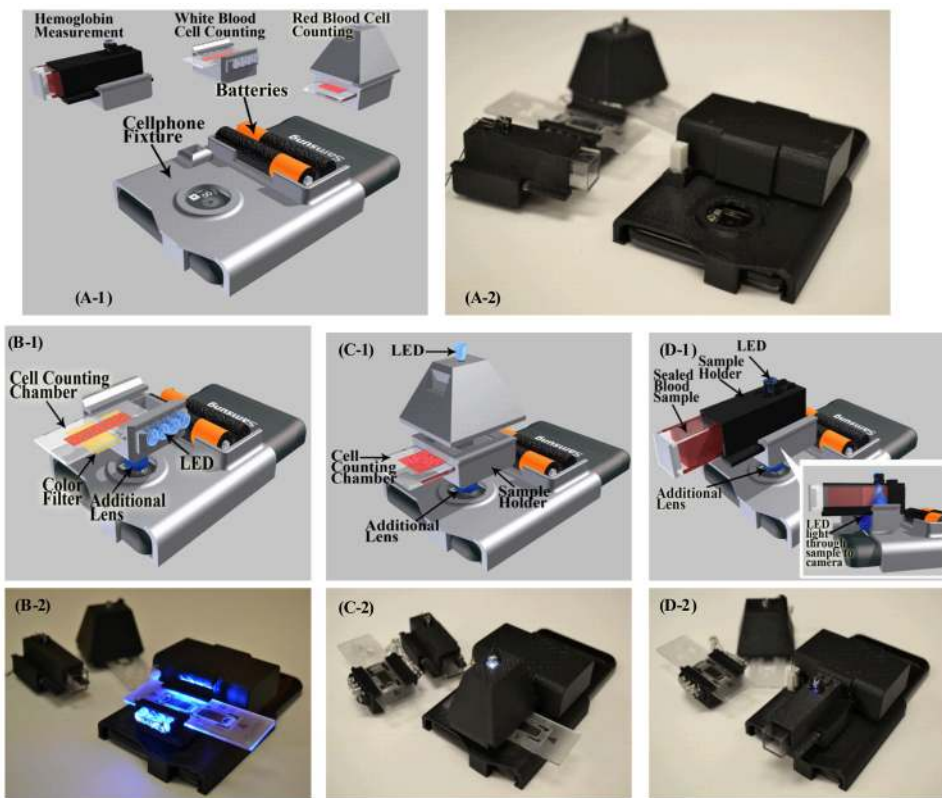
Figure 1. (A-1) and (A-2) Illustration and picture of our cell-phone based blood analysis platform. It includes a base attachment with two AA batteries and a universal port for adapting three different add-on components for white blood cell counting, red blood cell counting and hemoglobin measurements respectively. (B-1) and (B-2) Illustration and picture of the white blood cell counting device. (C-1) and (C-2) Illustration and picture of the red blood cell counting device. (D-1) and (D-2) Illustration and picture of hemoglobin measurement device.
