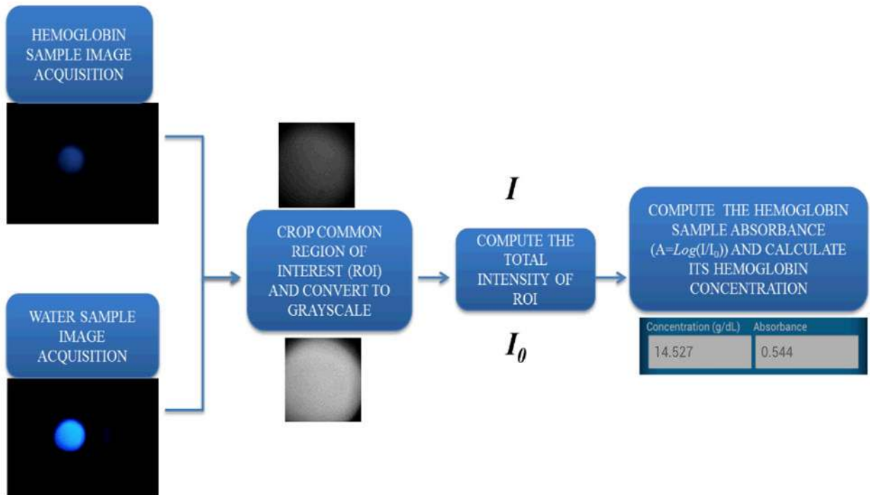
Figure 5. Block diagram of the digital processing steps that run on our cell-phone for hemoglobin concentration measurements.
