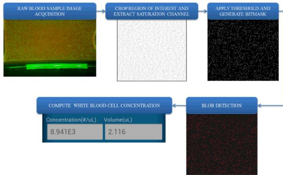
Figure 3. Block diagram of the digital processing steps that run on our cell-phone for white blood cell concentration measurements.
