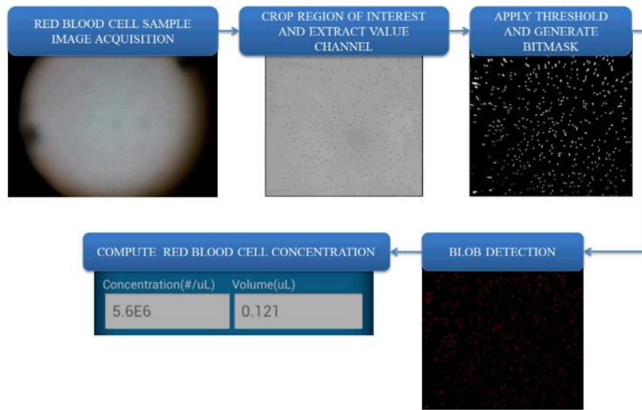
Figure 4. Block diagram of the digital processing steps that run on our cell-phone for red blood cell concentration measurements.
