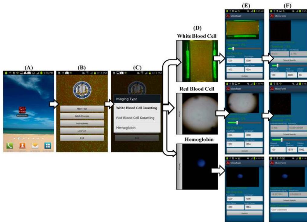
Figure 2. (A) “Blood analysis” icon on the cell phone home screen. (B) Once the user clicks on the “blood analysis” icon, the login screen pops up and the user can choose to start a new test. (C) When a new test is initiated, a test menu is shown and the user can choose the test type: white blood cell counting, red blood cell counting or hemoglobin measurement. (D) After the user chooses the test type, she/he can take the picture of the sample using the camera installed on the cell-phone. (E) The application displays a raw image of the test and the user can dynamically change the default values for the region of interest such as image pixel size, sample dilution factor and sample chamber depth. (F) After clicking the “Analyze” button, test results are displayed on the phone within a processing time of ~10 sec per test. The test results can then be stored at the cell-phone memory or be uploaded to a central database/ server.
