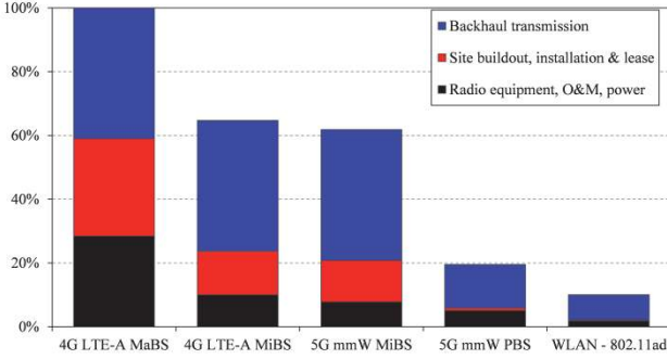
Fig. 1. BS discounted cost structure of AWA-HetNet.
