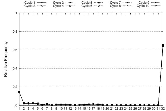
(b) Frequency that a given number of bits per architectural register are corrupted when faults are injected into logic
