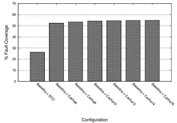
11: Fault coverage for a variety of register file configurations
