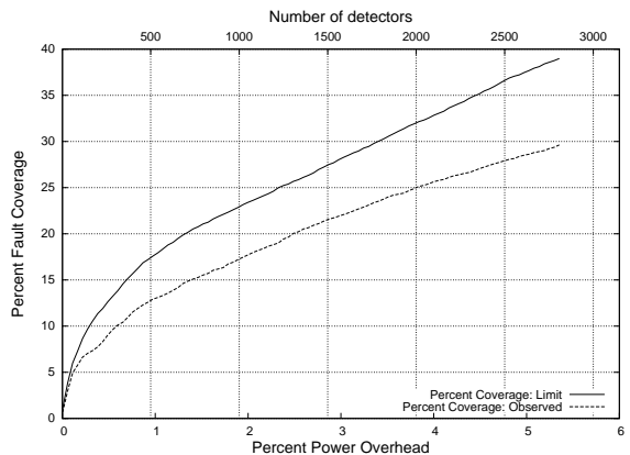
(b) Percent power overhead for transient fault detection units. The secondary x axis shows the number of detectors (i.e. the number of flip-flops augmented with detection units)
